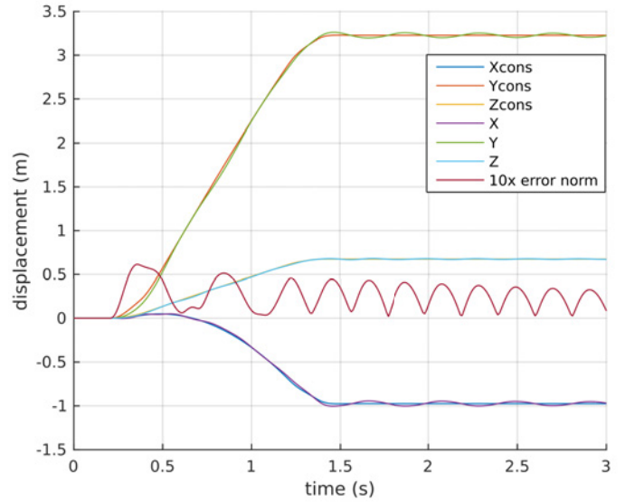
FIGURE 8. EOA TRAJECTORY TRACKING ERROR
