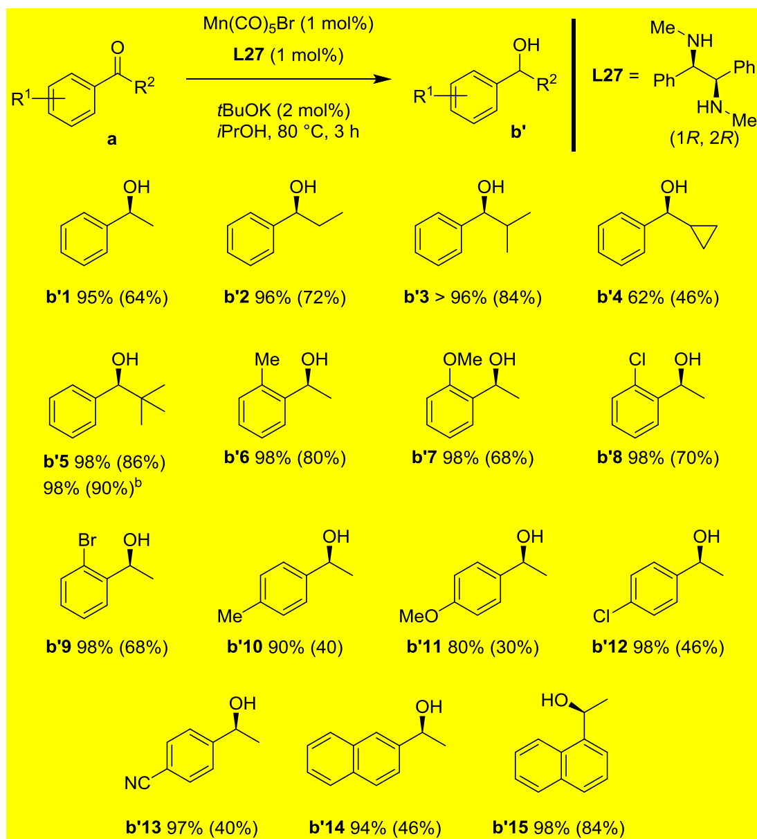
Scheme 4: Scope of the asymmetric reduction of ketones catalyzed by (1R, 2R) -(+)-N,N'-dimethyl-1,2-diphenyl-1,2-ethane diamine L27 and \text{Mn}(\text{CO})_5\text{Br} . a [ a Typical conditions : To a solution of ketone in 2-propanol were added in this order the diamine (1 mol%), \text{Mn}(\text{CO})_5\text{Br} (1 mol%) and finally t\text{BuOK} (2 mol%). Conversion determined by ^1\text{H} NMR, ee determined by chiral GC given in parentheses. Each reaction has been repeated at least twice. b 50^\circ\text{C} , 24 h.]
