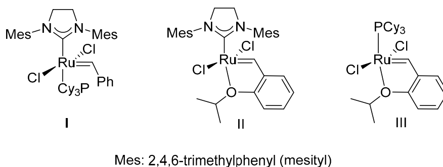
Figure 2. Ruthenium catalysts used in the screening experiments.
