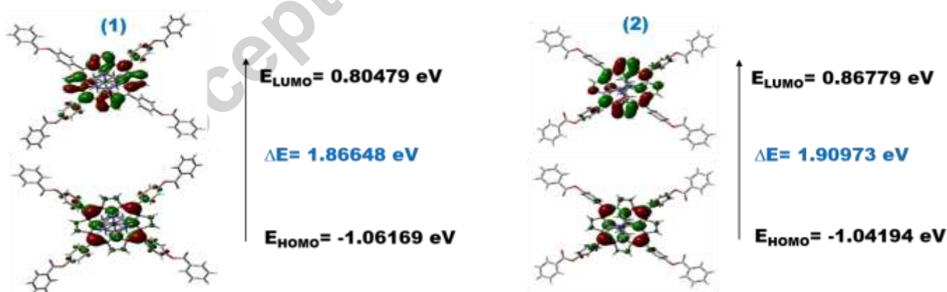
Fig. 11. Frontier molecular orbitals (HOMO and LUMO) plots of (1) and (2). Contour surfaces of orbital amplitude 0.02 (red) and -0.02 (green) are shown. (single-column figure)
