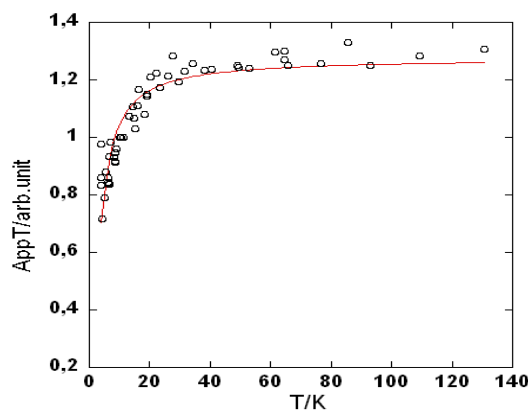
Figure 14. Temperature dependence of the product A_{pp}T in \text{CH}_2\text{Cl}_2 solution for 2\text{Cu}^+ complex.
