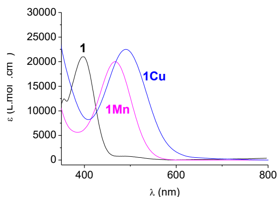
Figure 8. Electronic absorption spectra of 1 (black), 1Cu (blue), and 1Mn (magenta) in CH 2 Cl 2 .
