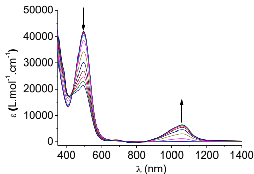
Figure 9. Electronic absorption spectra obtained upon the first oxidation of 2Cu in an OTTLE cell ( \text{CH}_2\text{Cl}_2 , 0.2 M \text{Bu}_4\text{NPF}_6 ).
