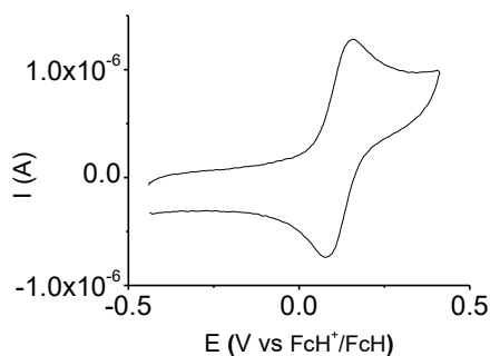
Figure 7. CV trace obtained for 1Cu in \text{CH}_2\text{Cl}_2 ( \text{Bu}_4\text{NPF}_6 , 0.1 M); \nu = 100 \text{ mV.s}^{-1} .
