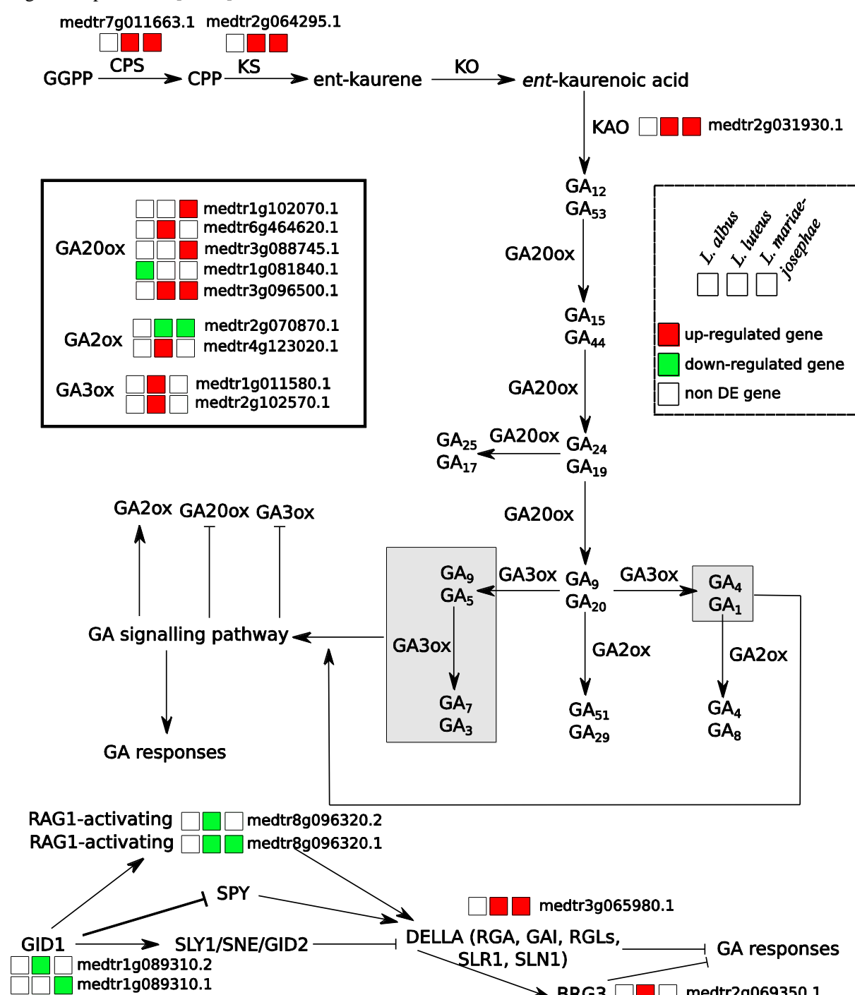
Figure 6: Gibberellins biosynthesis pathway and downstream regulation of GAs responses. For each gene, lupine species L. albus , L. luteus and L. mariae-josephae are respectively represented by the first, second and third squares. Squares are filled according the gene expression pattern as indicated in the top-right dashed rectangle: dark filling (red) stands for up-regulated genes (induced by compatible strains), light filling (green) for down-regulated genes (induced by incompatible strains) and white for not differentially expressed genes between the compatible and the non-compatible symbiotic situations. For each gene, the M. truncatula ortholog ID is indicated. Grey boxes indicate the biologically active forms of GAs. Expression pattern of genes encoding GA20ox, GA3ox and GA2ox are indicated in the dashed square. Figure adapted from [89,90].
