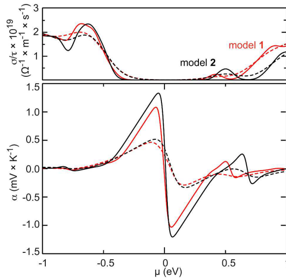
Fig. 3 Electrical conductivity ( \sigma/\tau ) and Seebeck coefficient ( \alpha ) computed as a function of chemical potential ( \mu ) for \text{Ag}_4\text{Mo}_9\text{Se}_{11} models at 300 K (plain) and 800 K (dotted).
