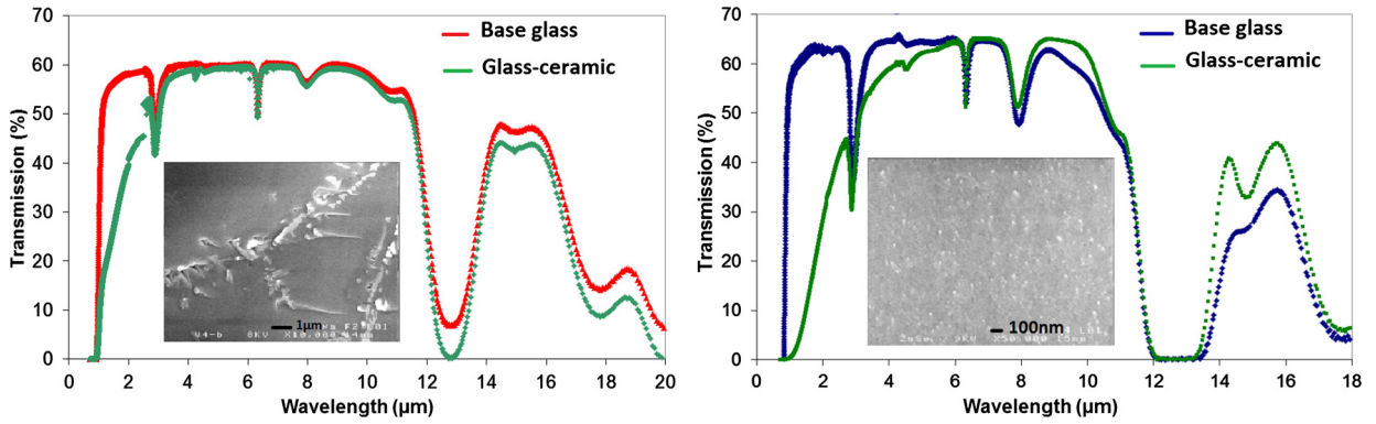
Fig. 6. (a) 73\text{GeSe}_2\text{-}20\text{Sb}_2\text{Se}_3\text{-}7\text{CdTe} glass and glass-ceramic (annealed at 290\text{ }^\circ\text{C} for 5 h). Inset: a SEM picture of the obtained particles. (b) Transmission of 70\text{GeSe}_2\text{-}20\text{Sb}_2\text{Se}_3\text{-}5\text{ZnSe} glass and glass-ceramic annealed at 340\text{ }^\circ\text{C} for 5 h. Inset: SEM picture of the obtained nanoparticles.
