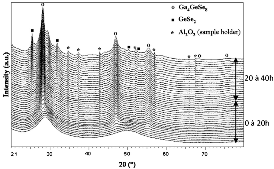
Fig. 7. X-ray diffractograms of the 80\text{GeSe}_2\text{-}20\text{Ga}_2\text{Se}_3 glass annealed at 380\text{ }^\circ\text{C} for 40 h. Reprinted from [10].
