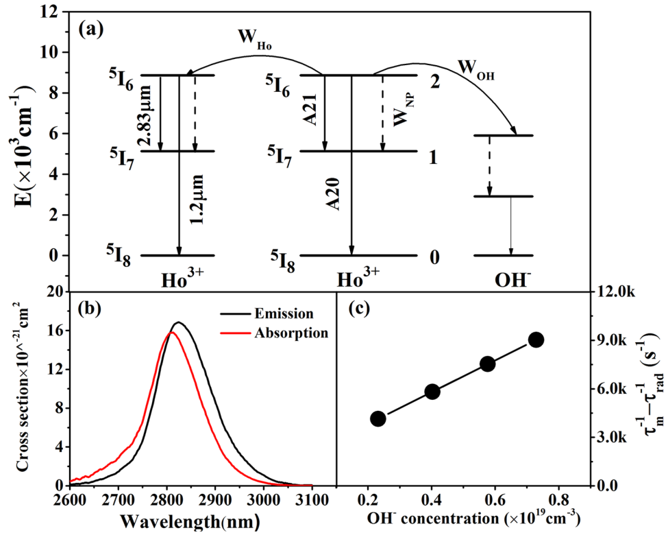
Figure 6. (a) Radiation transition and nonradiation transition processes of Ho^{3+} in the fluorotellurite-germanate glass; (b) Overlaps of absorption and emission cross-section spectra of the 2.83 \mu m band; (c) \tau_m^{-1} - \tau_{rad}^{-1} as a function of OH^- concentration.
