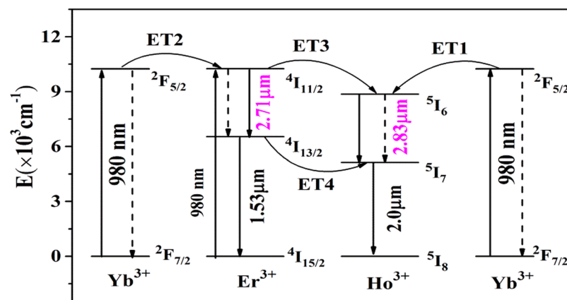
Figure 4. Energy level schemes and energy transfer processes between Ho 3+ , Er 3+ and Yb 3+ .
