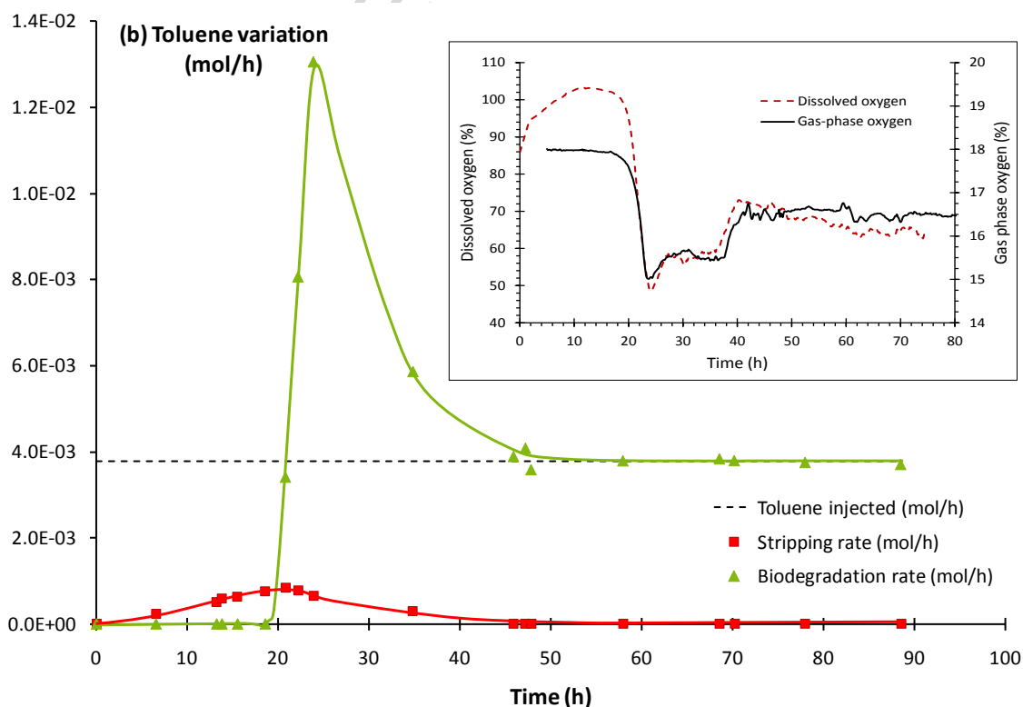
(b) derivative curves corresponding to the stripping and biodegradation rates. Insert: oxygen measurements
