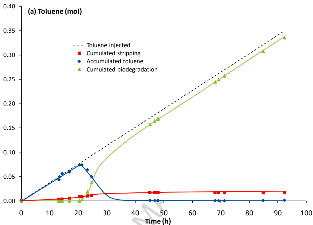
(a) mass balance of the amount of injected toluene between stripping, biodegradation and accumulation in the water/PDMS 50 mixture
