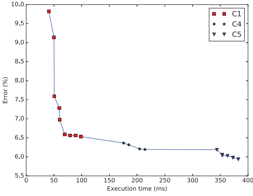
Figure 16: Latency and quality of the best solutions
