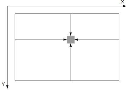
Figure 4: aggregation paths
