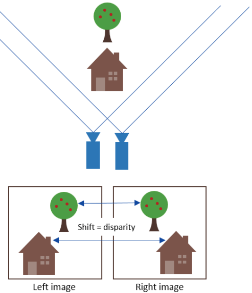
Figure 1: Disparity in stereoscopic images
