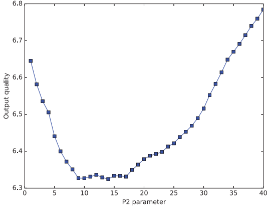
Figure 8: SGM P2 parameter variation.
