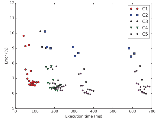
Figure 15: Speed and quality of different solutions
