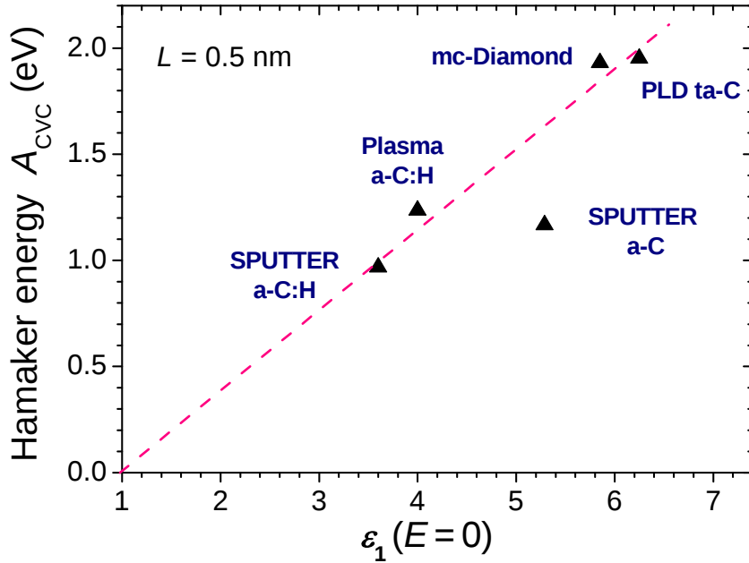
Fig. 6. Calculated A_{CVC} Hamaker energy for a-C and mc-diamond films, showing a linear correlation with the real dielectric function in the IR range (Eqn. 21).
