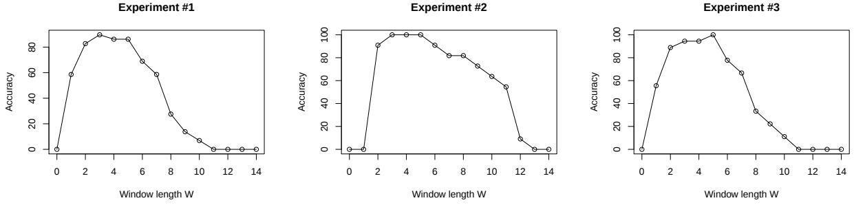
Figure 6: Evolution of the accuracy according to the window length.
