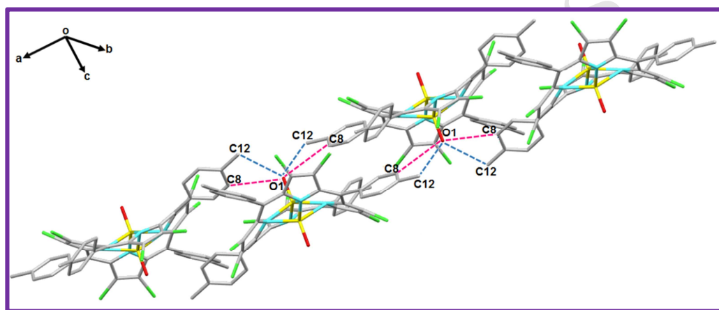
Figure 6. A partial view of the crystal packing of ( I ) showing the links within one layer between the [\text{V}(\text{Cl}_8\text{TTP})\text{O}] complexes via non-classical \text{C}-\text{H}\cdots\text{O} hydrogen bond.
