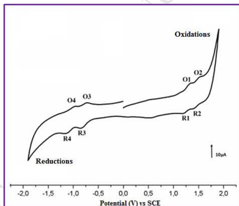
Figure 2. Cyclic voltammogram of [\text{V}(\text{Cl}_8\text{TTP})\text{O}] ( I ). The solvent is \text{CH}_2\text{Cl}_2 , the concentration is ca. 10^{-3} M in 0.2 M \text{TBAPF}_6 , the scan rate is 100 mV/s, vitreous carbon working electrode ( \varnothing = 3 mm).
