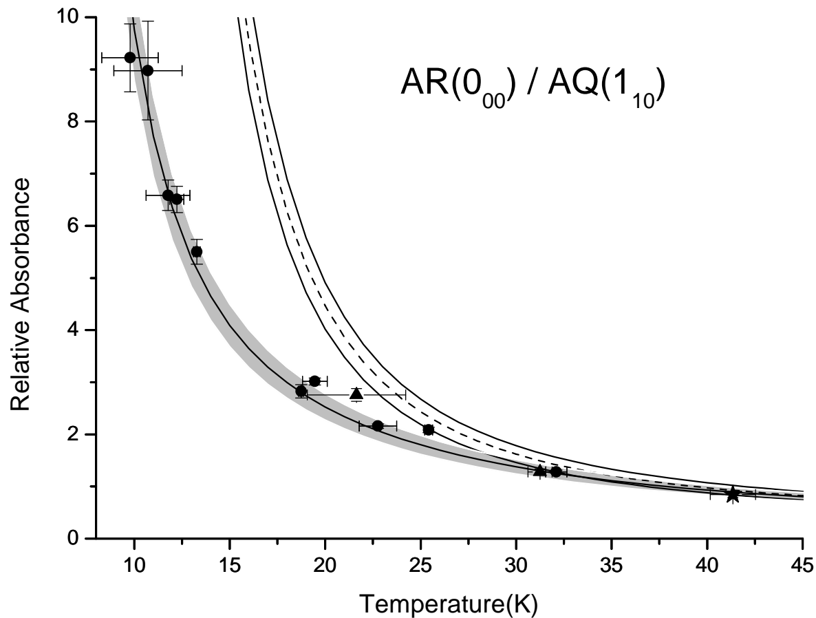
Figure 9: Relative integrated absorbances A_{1_{01} \leftarrow 0_{00}} / A_{1_{11} \leftarrow 1_{10}} measured as a function of rotational temperature. See Fig. 7 caption for more details.
