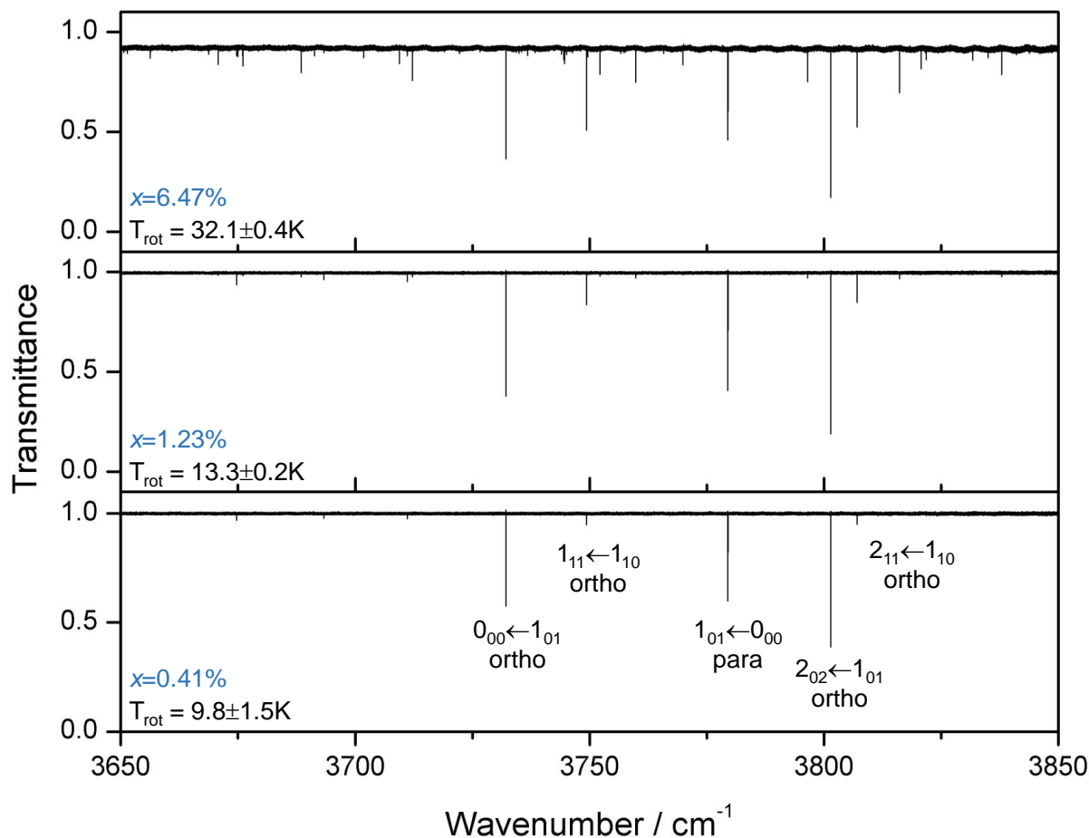
Figure 1: Selection of jet-cooled transmittance spectra recorded at 0.002 \text{ cm}^{-1} resolution to avoid line saturation effects. Water clustering, driven by the partial pressure of water vapor present in the flow, is one of the means used to control the temperature of the flow (argon in these examples). Rotational temperature increases from the lower to the upper panel as the water molar fraction increases. In our study, relative intensities were calculated using four ortho transitions (given using the notation “band \nu_3 \leftarrow ground state” by: 2_{02} \leftarrow 1_{01} ; 0_{00} \leftarrow 1_{01} ; 1_{11} \leftarrow 1_{10} ; 2_{11} \leftarrow 1_{10} ) and one para transition ( 1_{01} \leftarrow 0_{00} ).
