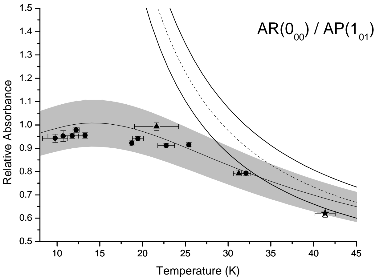
45 46 47 48 49 50 51 52 53 54 55 56 57 58 59 60 Figure 8: Relative integrated absorbances A_{101 \leftarrow 000} / A_{000 \leftarrow 101} measured as a function of rotational temperature. See Fig. 7 caption for more details.
