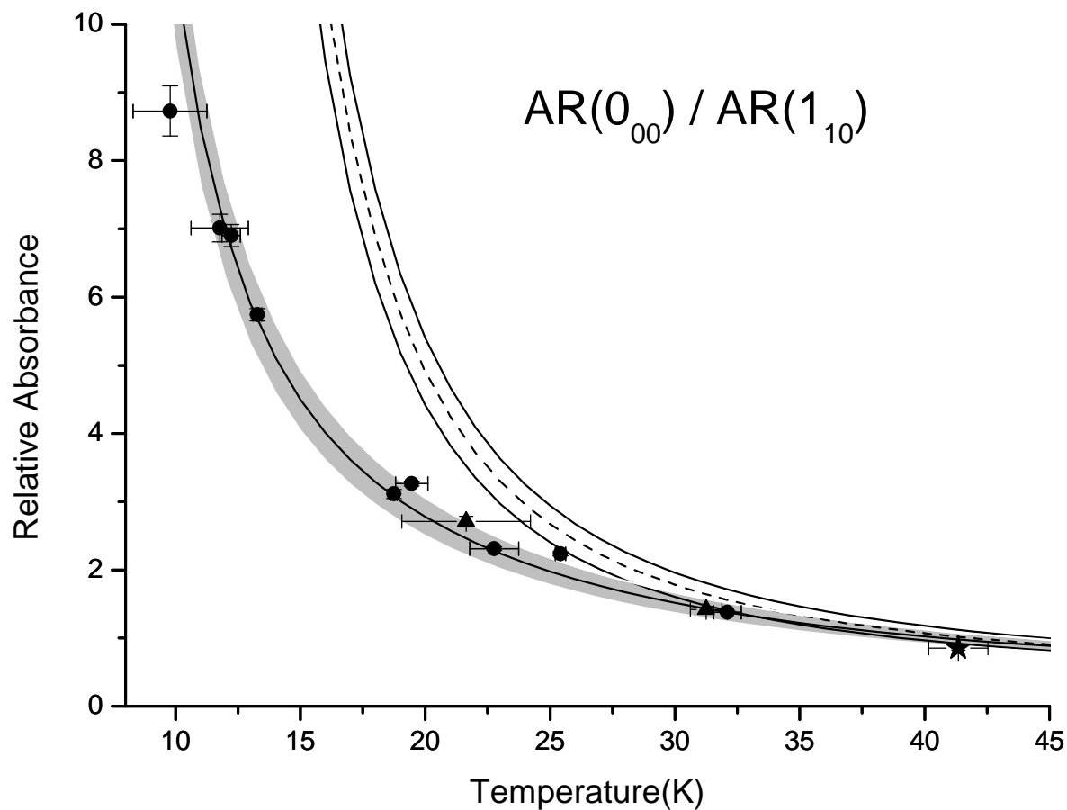
Figure 10: Relative integrated absorbances A_{1_{01} \leftarrow 0_{00}} / A_{2_{11} \leftarrow 1_{10}} measured as a function of rotational temperature. See Fig. 7 caption for more details.
