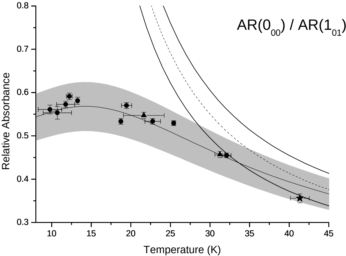
Figure 7: Relative integrated absorbances A_{1_{01} \leftarrow 0_{00}} / A_{2_{02} \leftarrow 1_{01}} measured as a function of rotational temperature. The expected behaviour in case of Slow NSC (solid line) and in case of Fast NSC (dashed line) is also represented. The uncertainty of 10% on the theoretical values are shown in gray are derived from HITRAN 32 data. Triangle symbols represent data obtained in pure oxygen or in a mixture with equal Ar and O 2 flow rates as a carrier gas, as shown in Table 3, whereas the star refers to the data obtained in an expansion of He instead of Ar as a carrier gas. The x-axis error bars reflect the uncertainty of the rotational temperature retrieved from the rotational diagram. The y-axis error bars originate from the most severe estimate of uncertainty in the line intensities measurements following subtraction, when possible, of the hot gas contribution to the low-temperature line absorption.
