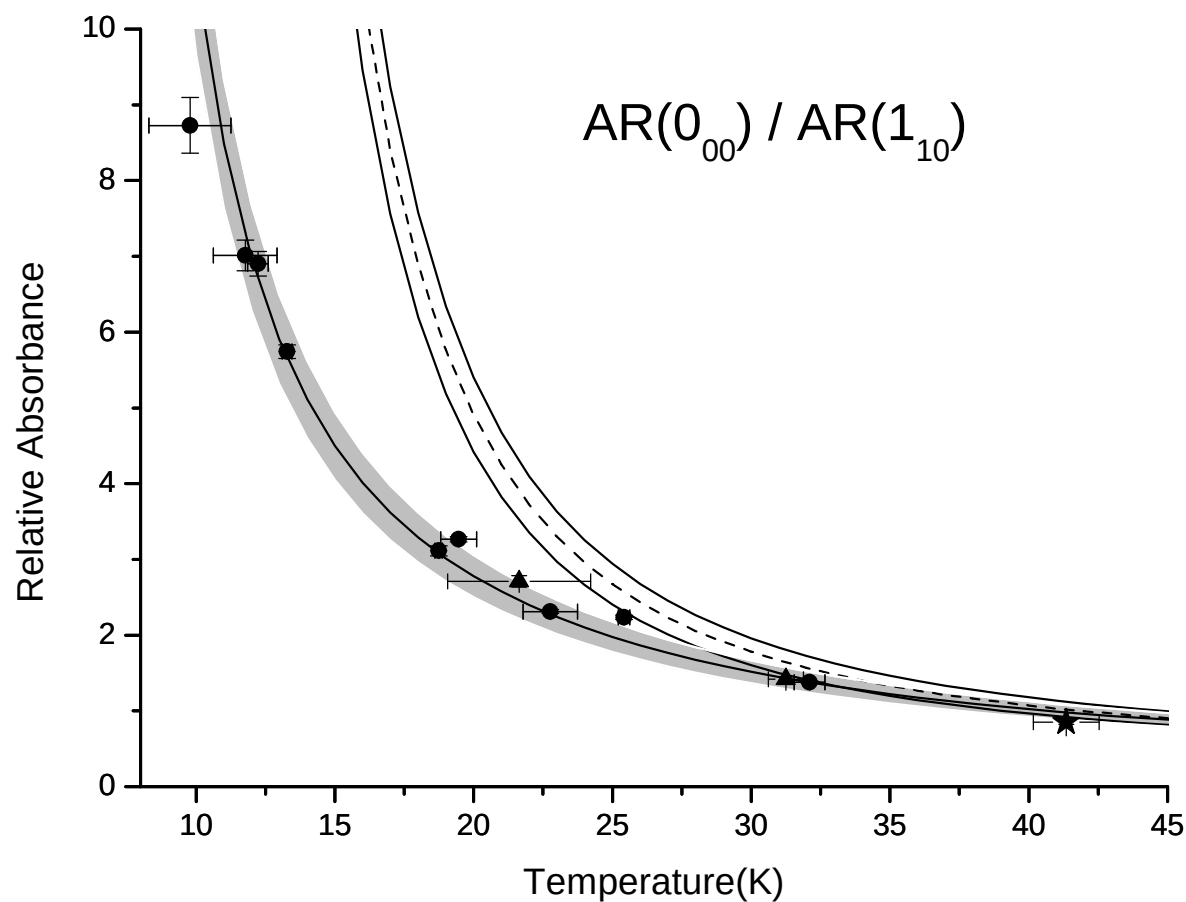
Figure 10: Relative integrated absorbances A_{1_{01} \leftarrow 0_{00}} / A_{2_{11} \leftarrow 1_{10}} measured as a function of rotational temperature. See Fig. 7 caption for more details.
