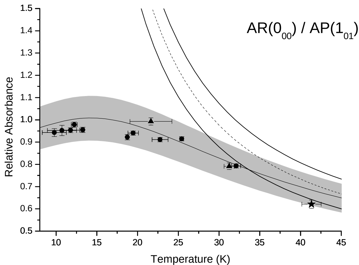
Figure 8: Relative integrated absorbances A_{1_{01} \leftarrow 0_{00}} / A_{0_{00} \leftarrow 1_{01}} measured as a function of rotational temperature. See Fig. 7 caption for more details.
