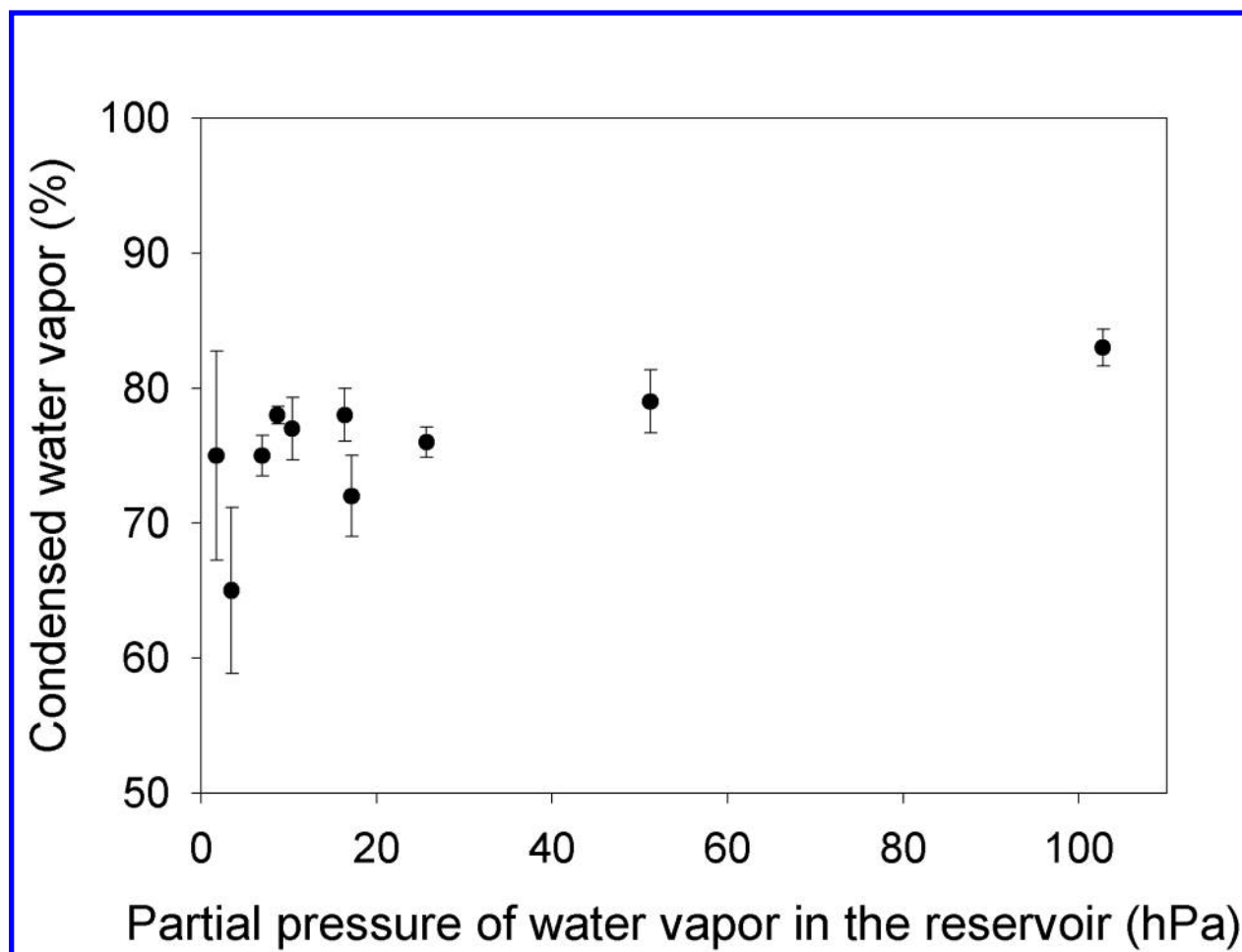
Figure 4: Concentration of condensed water vapor in an expansion of argon. These values, estimated from the measured monomer absorption, reveal a strong water condensation (between 65 and 83 %) even for small partial pressures of water vapor.
