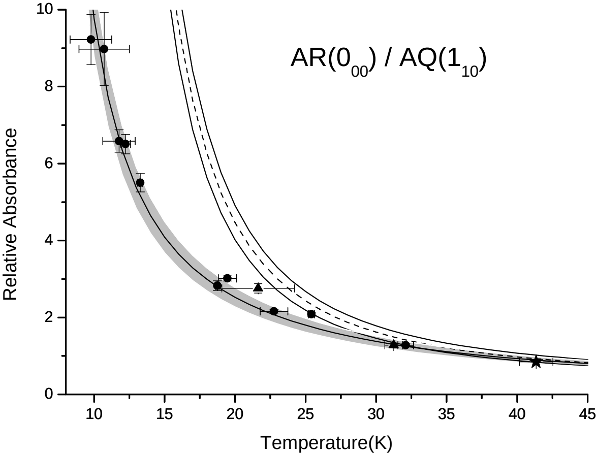
Figure 9: Relative integrated absorbances A_{1_{01} \leftarrow 0_{00}}/A_{1_{11} \leftarrow 1_{10}} measured as a function of rotational temperature. See Fig. 7 caption for more details.
