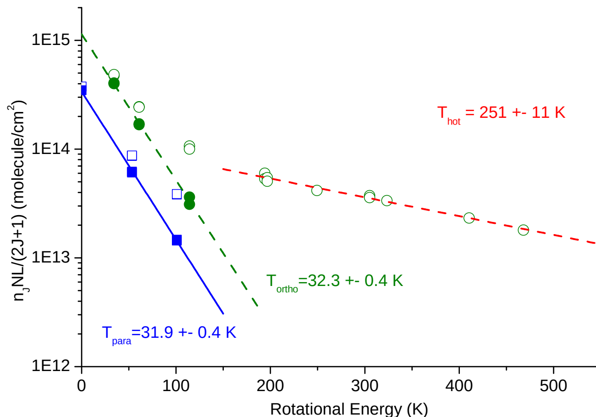
Figure 5: Example of rotational diagram used to extract the rotational temperature from absorbance spectra in the case of the presence of hot and cold molecules in the path of the infrared beam (here 100 g/h of H 2 O in 30 slm of Argon). The quantity (N L n_i / (2J + 1)) (see Eq. 10) extracted from the fitting of the different lines, is represented as a function of the energy level E_i of the initial state of the transition. The open circles and open squares represent the data obtained with a single Gaussian profile for ortho and para lines respectively. The data for energies E_i higher than 190 K follow a straight line and the slope gives the rotational temperature of the hot molecules ( 251 \pm 11 \text{ K} ). The warm gas contribution is then removed from the low- J rotational line absorption by a fitting procedure taking into account the hot and cold contributions (see text for details), leading to a corrected value of the cold gas rotational temperature for the ortho molecules ( 32.3 \pm 0.4 \text{ K} ) very close to the rotational temperature extracted from the lines associated with the para molecules ( 31.9 \pm 0.4 \text{ K} ). A total of 8 low- J rotational lines have been used to estimate the cold rotational temperature.
