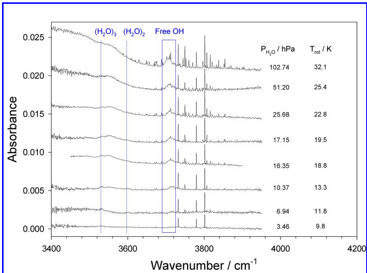
Figure 2: Series of low resolution absorbances (offset for clarity) of water vapor cooled in argon (400 co-added scans at 1 \text{ cm}^{-1} resolution). Water clustering is driven by the water vapor partial pressure (as indicated in the rightmost part of the figure) in the stagnation reservoir. In addition to the partially resolved water monomer lines, both the signatures of free OH (around 3710 \text{ cm}^{-1} ) and bound OH vibrations are observed. 20 The signatures of the water dimer and trimer can be seen at 3601 and 3533 \text{ cm}^{-1} , respectively, for conditions leading to weak clustering. The broad absorption observed below 3600 \text{ cm}^{-1} , corresponds to much larger water clusters that form at enhanced water vapor partial pressure.
