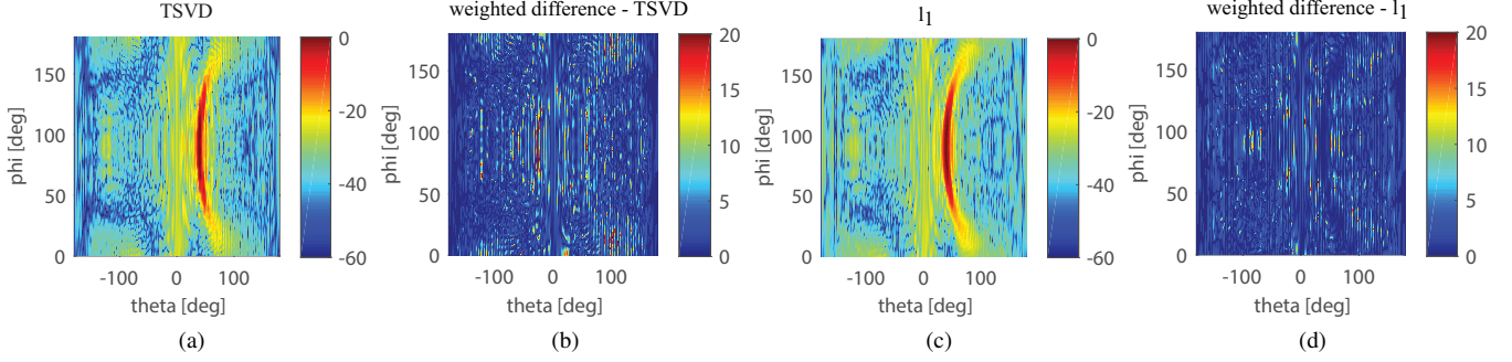
Fig. 11: 3D far field mappings in dB radiated by the plate Luneburg lens and interpolated from the ‘igloo’ sampling represented Fig. 10(a) M = 2057 points and for a truncation order of L = 55 , i.e. N = 3136 spherical modes. Far field pattern and weighted difference between exact and reconstructed field obtained (a,b) by the TSVD approach and (c,d) by the proposed the \ell_1 minimization procedure (5).
