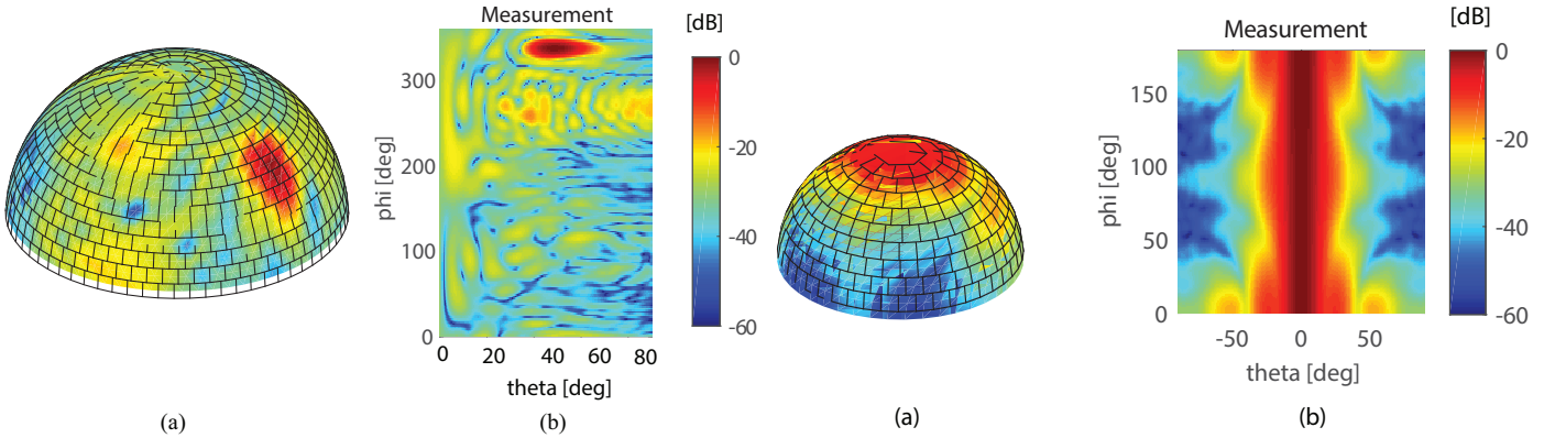
Fig. 7: Far field patterns radiated by the standard gain horn at 26 GHz: (a) sampling using the ‘igloo’ technique with \Delta\theta = 8^\circ ( M = 339 sampling points) and (b) measured 3D field mapping y_{\text{Meas}} .
