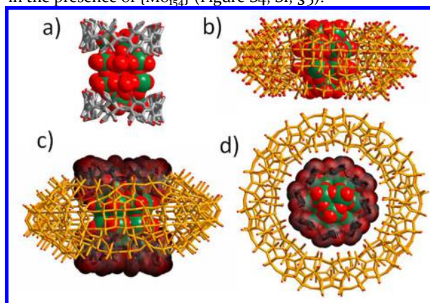
Figure 3. Mixed representations of the supramolecular hierarchical compound 1 [\{\text{P}_2\text{W}_{18}\text{O}_{62}\}@2\gamma\text{-CD}@{\text{Mo}}_{154}\} : a) highlight of the inner adduct built from a Dawson anion [\text{P}_2\text{W}_{18}\text{O}_{62}]^{6-} capped by two \gamma\text{-CD} tori. b) representation showing the deep inclusion of the Dawson anion within the large inner cavity of the Mo-blue ring-shaped anion. c) Side and d) Top views of the hybrid supramolecular adduct showing the hierarchical organization between three components with the Dawson anion at the center (green and red space-filling spheres) capped by two \gamma\text{-CD} (wires and transparent space-filling spheres) encaged into the large \{\text{Mo}_{154}\} torus (yellow sticks).
