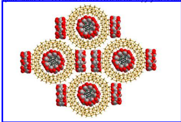
Figure 4. Selected view of 1 showing large holes delimited by the \{\text{Mo}_{154}\} packing which are filled by two outer \gamma -CD units.
