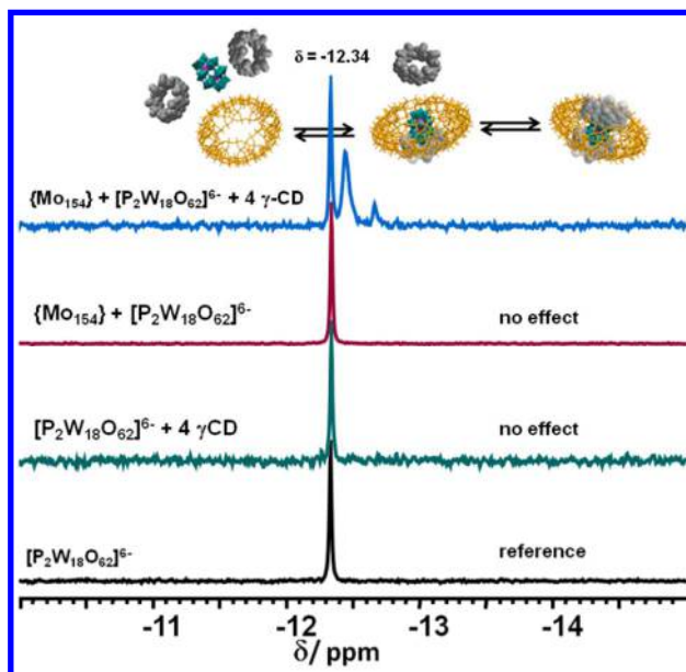
Figure 5. ^{31}\text{P} NMR spectrum of 1 (top) showing that only simultaneous presence of the three components provokes a clear change of ^{31}\text{P} NMR spectrum. The presence of four ^{31}\text{P} NMR signals with 32 : 52 : 8 : 8 intensity ratio is consistent with [\text{P}_2\text{W}_{18}\text{O}_{62}]^{6-} ion as solvated ion ( \delta = -12.34 ppm) or as central guest species into the three-component assemblies ( \delta = -12.43 , -12.53 and -12.69 ppm). The presence of three shielded ^{31}\text{P} resonances should be interpreted as slow equilibria occurring between bicapped and monocapped guest species as depicted in scheme inserted on the upper ^{31}\text{P} NMR spectrum.
