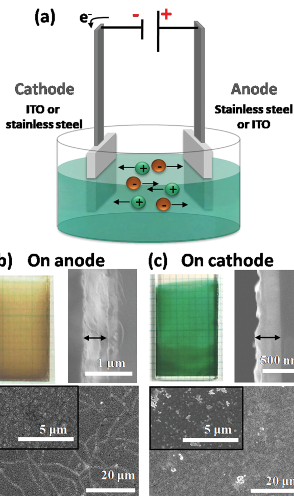
Fig. 2 (a) Schematic representation of anodic (ITO on the anode and stainless steel on the cathode) or cathodic (ITO on the cathode and stainless steel on the anode) EPD; (b) photograph and SEM images of the cross section and surface of the brown-Ta 6 @ITO film (25 V and 60 s); (c) photograph and SEM images of the cross section and surface of the green-Ta 6 @ITO film (20 V and 60 s).
