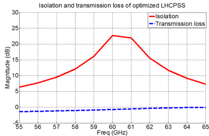
Figure 8. Isolation and transmission loss of optimized LHCPSS unit cell
