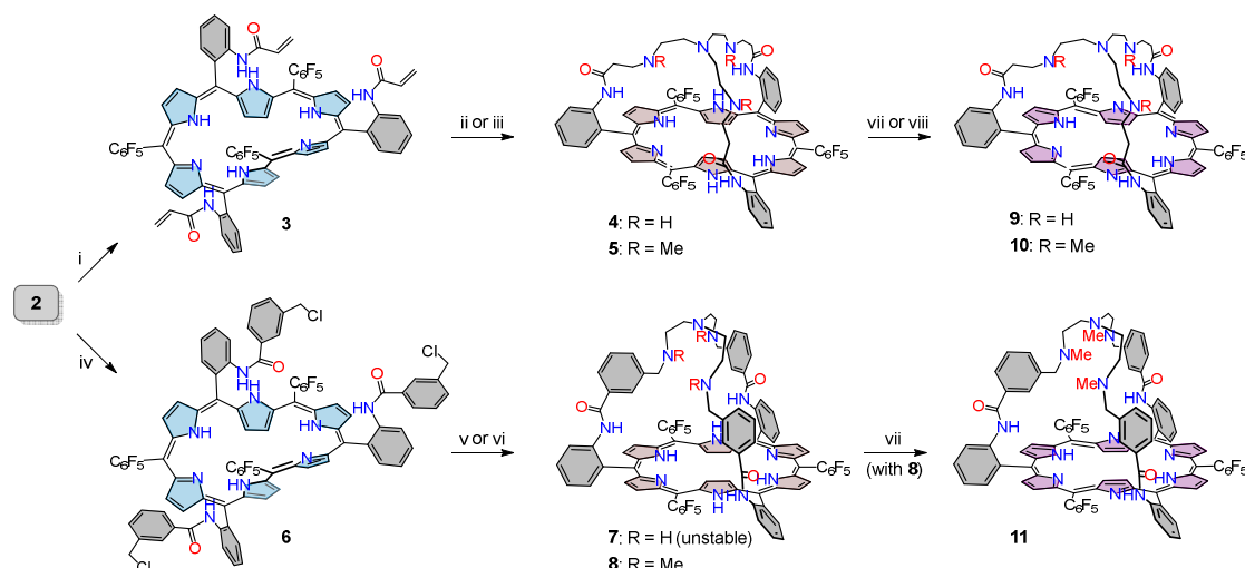
Scheme 2. Synthesis of tren-capped [28]hexaphyrins 4 , 5 , 7 , and 8 , and oxidation of compounds 4 , 5 and 8 in their 26\pi aromatic counterparts 9 , 10 and 11 . Conditions: i) acryloyl chloride, DIPEA, THF, -50^\circ\text{C} , 41 % (2 steps); ii) tren, \text{CHCl}_3/\text{CH}_3\text{OH} 1:9, 45^\circ\text{C} , 41 % ( 4 ); iii) Me-tren, \text{CHCl}_3/\text{CH}_3\text{OH} 1:9, 45^\circ\text{C} , 67 % ( 5 ); iv) 3-(chloromethyl)benzoyl chloride, \text{Et}_3\text{N} , THF, 0^\circ\text{C} , 46 % (2 steps); v) NaI, DIPEA, THF, 70^\circ\text{C} then tren, not characterized ( 7 ); vi) NaI, DIPEA, THF, reflux then Me-tren, 50^\circ\text{C} , 55 % ( 8 ); vii) DDQ, \text{CDCl}_3/\text{CD}_3\text{OD} 9:1 or \text{CDCl}_3 ( 9 and 11 ); (viii) DDQ, \text{CHCl}_3 , 82 % ( 10 ).
