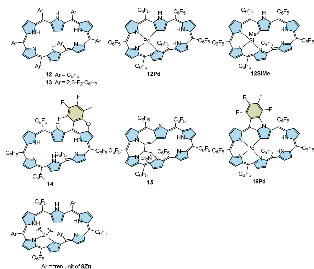
Chart 1. Selected Möbius aromatic hexaphyrins.
