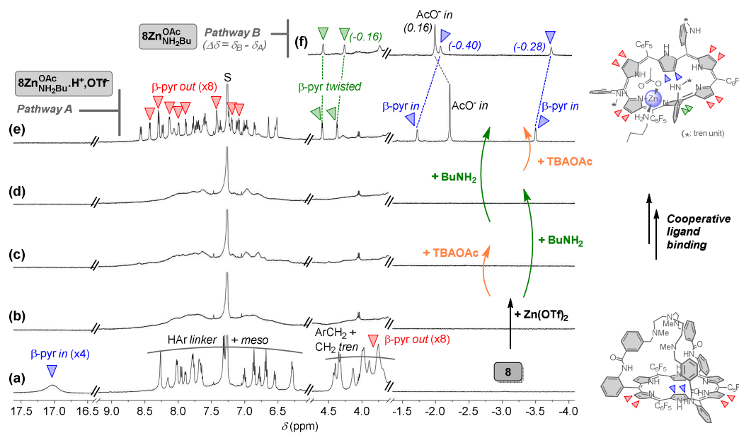
Figure 6. 1 H NMR study of the metallation of 8 with Zn(II) in two sets of conditions, namely pathway A (a-e) and pathway B (f) (CDCl 3 /CD 3 OD 9:1, 298 K, 500 MHz, selected regions). Conditions, pathway A: (a) 8 , (b) 8 + 1 equiv. Zn(OTf) 2 , (c) 8 + 1 equiv. Zn(OTf) 2 + 1 equiv. TBAOAc, (d) 8 + 1 equiv. Zn(OTf) 2 + 1 equiv. BuNH 2 , (e) 8 + 1 equiv. Zn(OTf) 2 + 1 equiv. TBAOAc + 1 equiv. BuNH 2 ; pathway B: (f) 8 + 3.5 equiv. Zn(OAc) 2 + 7 equiv. DIPEA + 3 equiv. BuNH 2 . S = solvent.
