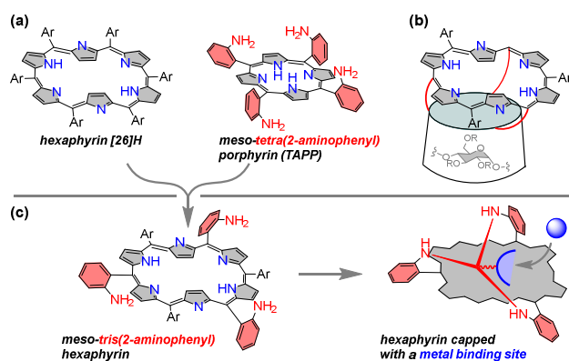
Figure 1. (a) Structures of the benchmark hexaphyrin [26]H and of the widespread TAPP platform. (b) Unique example of a triply-bridged hexaphyrin-cyclodextrin hybrid. (c) Global strategy of the present study to access first an hexaphyrin platform, and second hexaphyrins capped with a tripodal metal binding unit. Ar = C 6 F 5 .
