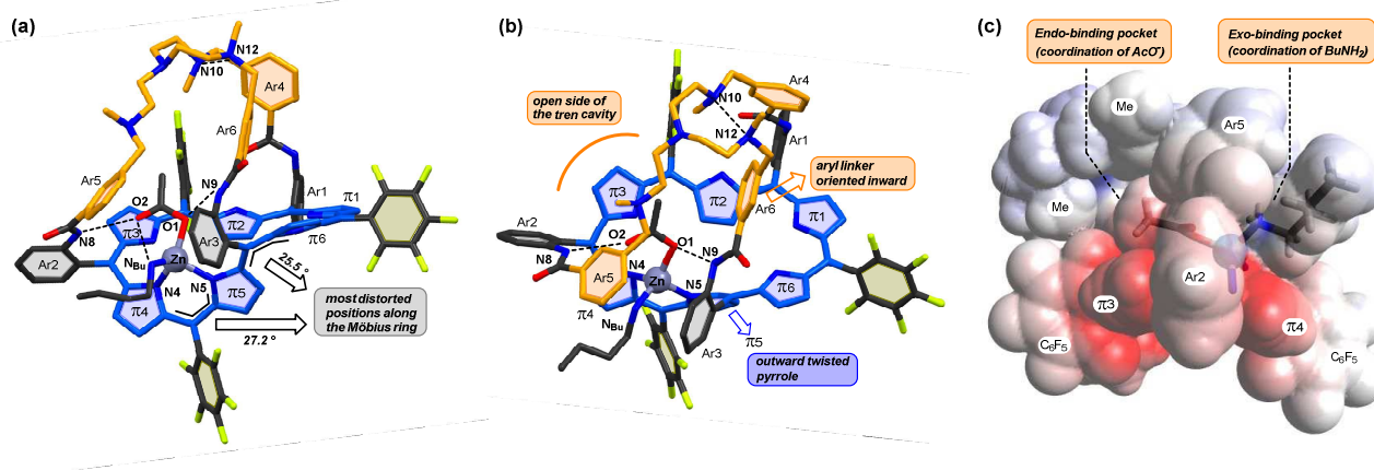
Figure 7. X-ray crystal structure of 8\text{Zn}^{\text{OAc}}\text{NH}_2\text{Bu}\cdot\text{H}^+\cdot\text{OTf} : (a) side and (b) top views (stick representation, hydrogen atoms, triflate counterion and solvents of crystallization have been removed for clarity; dashed lines indicate H-bonds). Blue: hexaphyrin part; orange: Me-tren- \text{CH}_2\text{Ar} unit. (c): perspective view from Ar2, highlighting the buried coordination site of Zn(II) affording endo - and exo -binding pockets (Van der Waals surface colored by electrostatic potential: blue/red for positive/negative potential; stick representation for the acetato and butylamino ligands, sphere representation for zinc). Selected distances (Å): N5-Zn 1.990, N4-Zn 2.044, \text{N}_{\text{Bu}} -Zn 2.049, O1-Zn 1.997, O1-N9 2.836, O2-N8 2.878, O2- \text{N}_{\text{Bu}} 3.062, N10-N12 2.949. Selected angles (°): O1-Zn-N5 103.07, O1-Zn-N4 120.34, O1-Zn- \text{N}_{\text{Bu}} 115.87, N5-Zn-N4 95.17, N5-Zn- \text{N}_{\text{Bu}} 115.42, N4-Zn- \text{N}_{\text{Bu}} 105.51. Dihedral angles along the SMC: see the SI.
