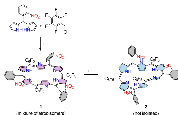
Scheme 1. Synthesis of hexaphyrin 2 . Conditions: i) MSA, CH 2 Cl 2 , 0 °C then DDQ, 16 %; ii) H 2 80 bars, Pd(0)/C (cat.), AcOEt, 30 °C.
