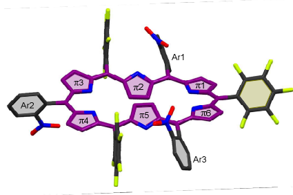
Figure 2. X-ray crystal structure of one atropisomer of 1 (stick view, hydrogen atoms and solvents of crystallization have been removed for clarity).
