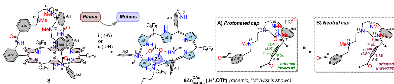
Scheme 3. Planar-to-Möbius topological change observed during Zn(II) metallation of 8 . Conditions (CDCl 3 /CD 3 OD 9:1, 298 K): i) 1 equiv. Zn(OTf) 2 , 1 equiv. TBAOAc, 1 equiv. BuNH 2 ; ii) 3.5 equiv. Zn(OAc) 2 , 7 equiv. DIPEA, 3 equiv. BuNH 2 ; iii) 10 equiv. DIPEA. Inset: chemical shift values (in parentheses) of the inward oriented aromatic moieties of a linker (Ar6).
