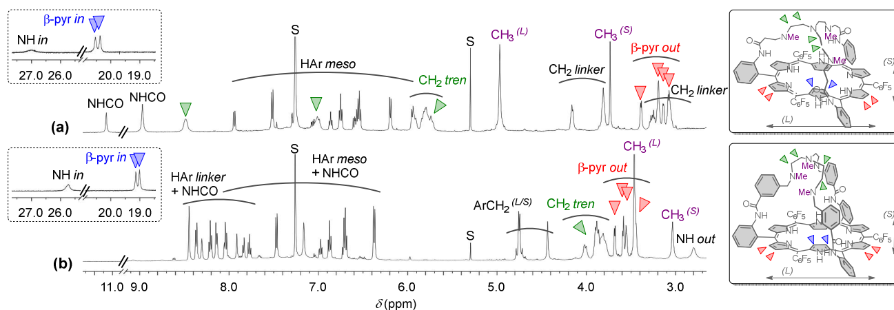
Figure 4. ^1\text{H} NMR spectra (selected parts) of 5 (a) and 8 (b) ( \text{CDCl}_3 , 298 K, 500 MHz). S = solvent; “L”/“S” italicized stand for “long”/“short”.
