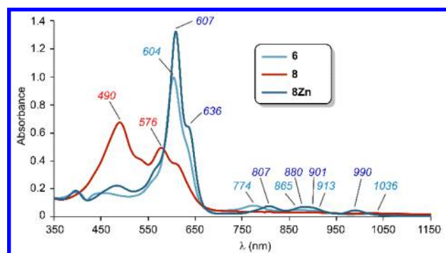
Figure 3. UV-vis-NIR absorption spectra of 6 ( \text{CH}_2\text{Cl}_2 ), 8 and 8Zn 0Ac NH 2 Bu (9:1 \text{CHCl}_3/\text{CH}_3\text{OH} ).
