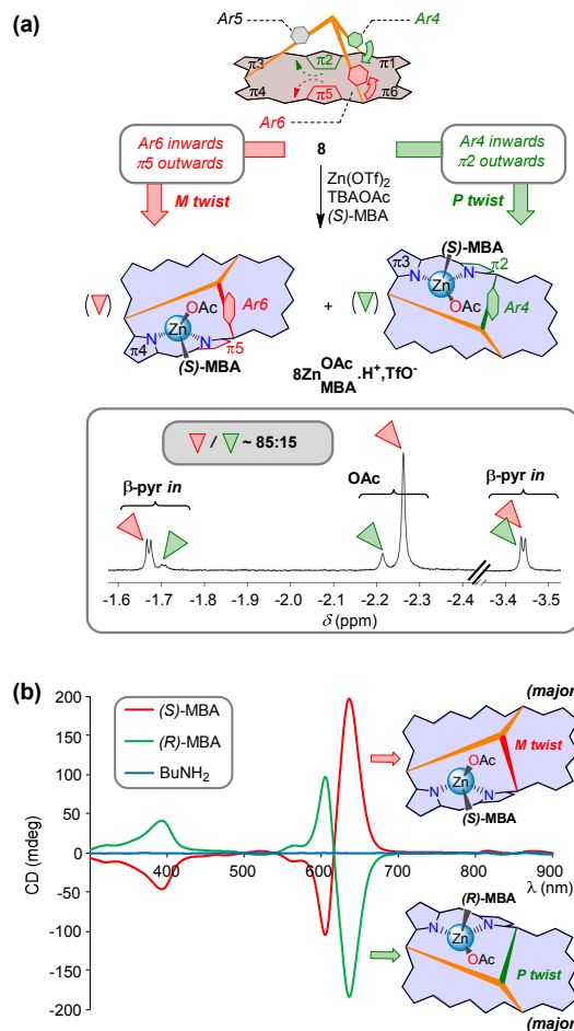
Figure 8. (a) Diastereoselective formation of Zn(II) Möbius complexes of 8 with ( S )-MBA and corresponding 1 H NMR spectrum (CDCl 3 /CD 3 OD 9:1, 276 K, highfield region). (b) CD spectra of 8Zn OAc RNH 2 .H + .OTf with RNH 2 = ( S )-MBA, ( R )-MBA or BuNH 2 (red, green and blue traces, respectively; initial concentration of 8 = 40 \mu M).
