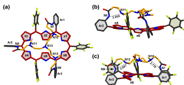
Figure 5. X-ray crystal structure of 5 : (a) top view; (b) and (c) side views from respectively the long side and the short open side (stick representation, hydrogen atoms have been removed for clarity). Brown: hexaphyrin part; orange: Me-tren- \text{CH}_2\text{CH}_2 unit. Dashed lines: H-bonds with distances in Å.
