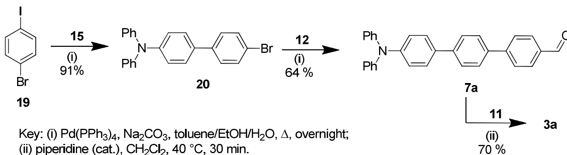
Scheme 4. Synthesis of 3a .
