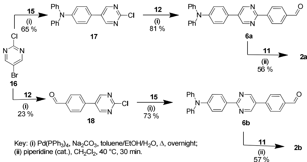
Scheme 3. Synthesis of 2a–b .
