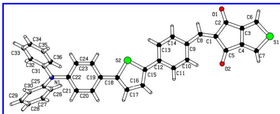
Figure 1. X-ray molecular representation of chromophore 3d (150 K, R = 0.05, CCDC 1549497).
