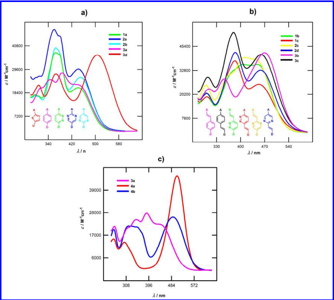
Figure 5. UV-Vis spectra of chromophores 1–4 measured in chloroform ( c \sim 10^{-5} M).
