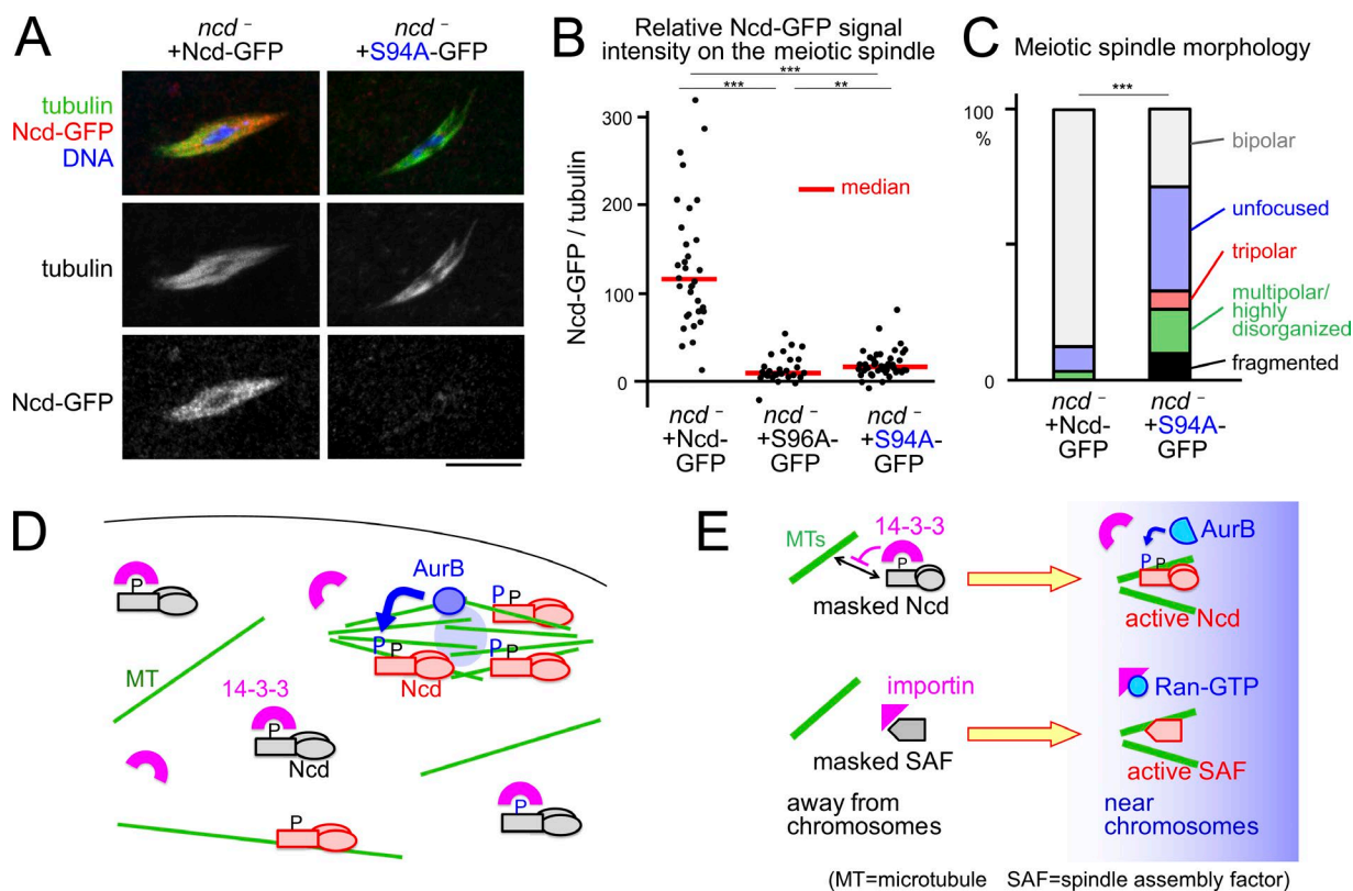
Figure 5. Aurora B phosphorylation is important for targeting Ncd to the spindle and spindle bipolarity. (A) Immunostaining of spindles in ncd l mutant oocytes carrying one Ncd-GFP transgene or one Ncd(S94A)-GFP transgene. Images were captured and modified using an identical setting. Bar, 10 \mu m. (B) GFP signal intensity relative to \alpha -tubulin signal on the spindle. n = 34, 27, and 41 . **, P < 0.01 ; ***, P < 0.001 . Note that these were imaged using a different microscope to Fig. 2. (C) Spindle morphologies in oocytes. n = 31 and 42 . (D and E) Aurora B (AurB) releases Ncd from 14-3-3 inhibition in oocytes analogously to the Ran–importin system, enabling Ncd to specifically bind spindle microtubules.
