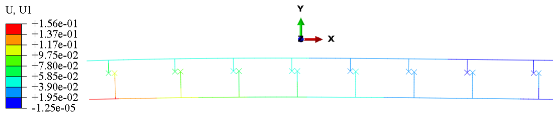
Figure 25: Simplified model: deformation (in mm)
