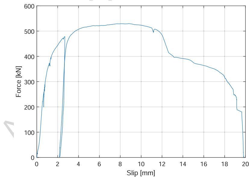
Figure 21: Residual resistance push-out test: force-slip curve
