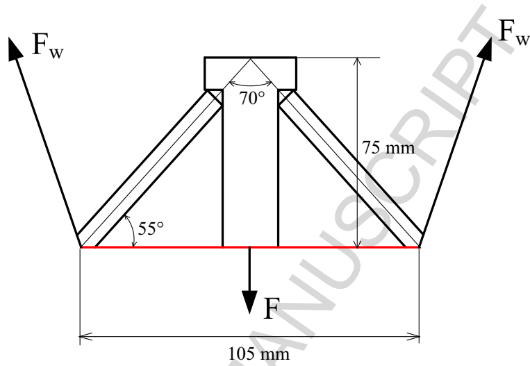
Figure 30: Strut and tie model
