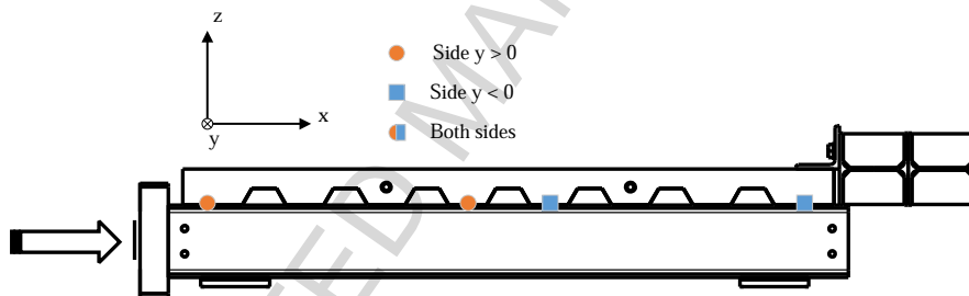
Figure 9: LVDT sensors: residual ultimate resistance test
