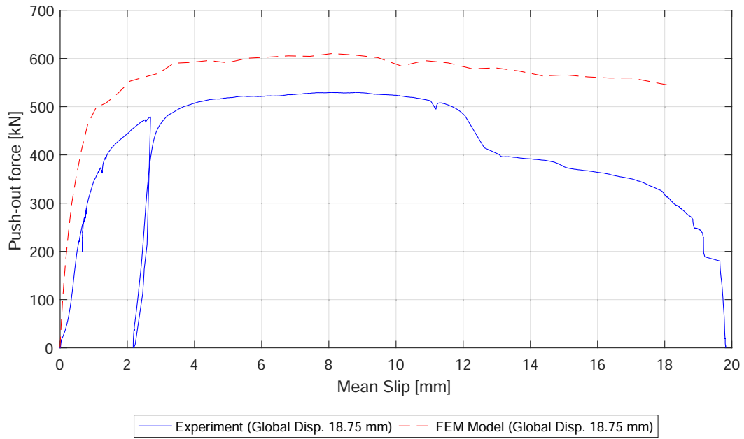
Figure 32: Comparison of residual ultimate load between experimental test and FEM simulation
