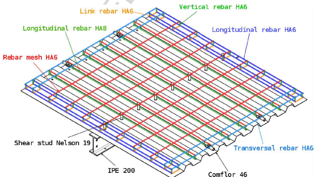
Figure 5: Composite beam specimen
