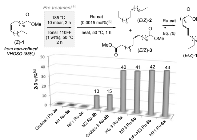
Figure 5. Screening of commercially available catalysts Ru-2-3 and Ru-5-6 in the SM of non-refined MO (Z)-1. [a] Conditions: 185 °C, 10 mbar, 2 h then sorbent (1 wt%), 50 °C, 2 h. [b] Conditions: Ru-catalyst (0.0015 mol%), 50 °C, neat, 1 h. [c] Percentage per weight of 2/3 in the crude, determined by GC (see ESI).
