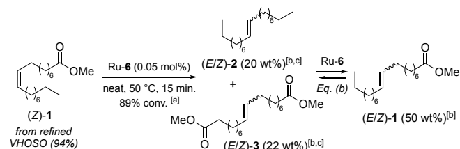
Scheme 2. Self-metathesis of MO (Z)-1 derived from refined VHOSO (94% of purity) catalyzed by SIPr-M71 Ru-6a. [a] Conversion of (Z)-1, monitored by GC (see ESI for details). [b] Percentage per weight of the composition of the crude at the equilibrium, determined by GC (see ESI). [c] E/Z ratio = 4/1.
