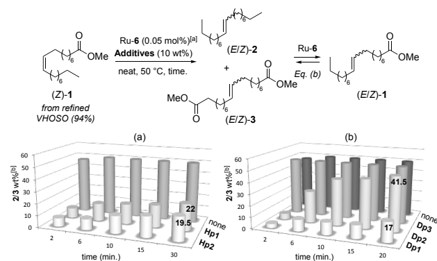
Figure 3. Kinetic profiles of the SM of MO (Z)-1 catalyzed by Ru-6a in presence of additives Hp (a) and Dp (b). [a] Conditions: Ru-6a (0.05 mol%), additive (10 wt%), 50 °C, neat. [b] Percentage per weight of 2/3 in the crude, determined by GC (see ESI).
