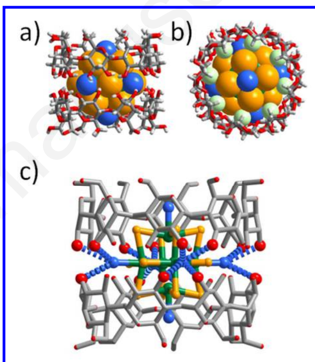
Figure 3. Mixed representations of the solid state structure of the supramolecular host-guest \{[Ta_6Br_{12}(H_2O)_6]@2\gamma\text{-CD}\}^{2+} complex : a) side view and b) top view highlighting close interactions between inner H-3 hydrogen (white sphere) and four bromide ligands (yellow sphere) with H\cdots Br = 2.83 Å; c) focus on the intermolecular hydrogen bonding network involving the four in plane aquo ligands of the cluster and the hydroxo groups of \gamma -CD secondary faces ( O\cdots O = 3.0 - 3.1 Å).
