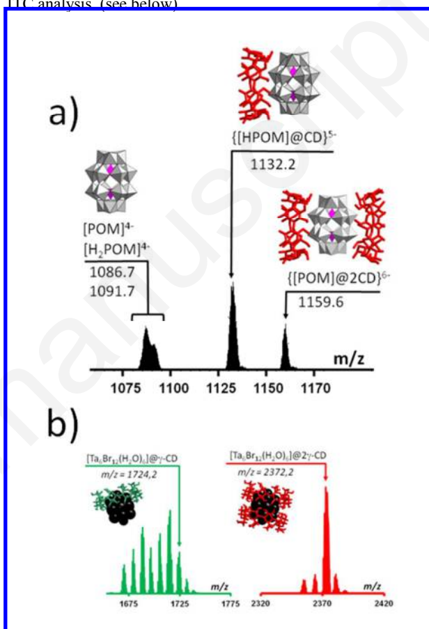
Figure 6. ESI-MS spectra of the inclusion compounds in aqueous solution. (a) \text{POM}@3\text{CD} showing the 1:1 and the 1:2 adducts while the 1:3 complex is not observed. (b) \{\text{Ta}_6\}@2\text{CD} containing the m/z peak related to the 1:2 (red trace) and 1:1 (green trace) adducts. The side peaks separated from each other by m/z = 9 are unambiguously attributed to either hydrated or dehydrated complexes.
