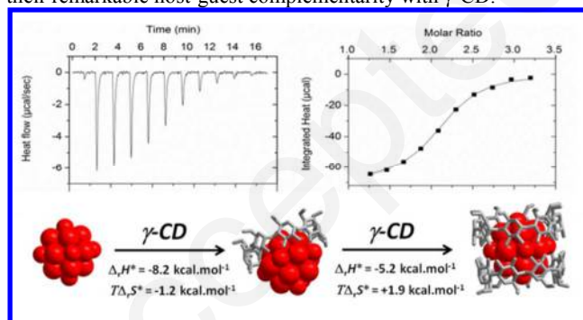
Figure 7. Microcalorimetric titration data obtained at 298 K from sequential injections of 3.33 mM \gamma -CD solution into a 0.33 mM [Ta_6Br_{12}(H_2O)_6]Br_2 solution showing ITC thermogram (left) and isotherm (right). Dots and full lines correspond to experimental and calculated heats obtained from thermodynamic parameters describing a two-step sequential binding process (bottom).
