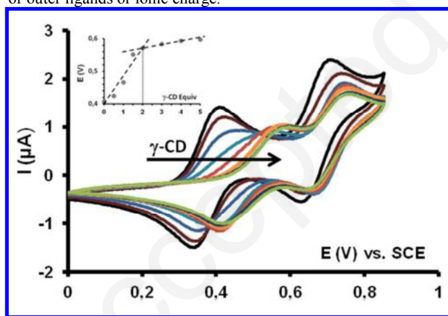
Figure 8. Cyclic voltammograms of [\text{Ta}_6\text{Br}_{12}(\text{H}_2\text{O})_6]^{2+} (0.5mM, 298K, scan rate 10\text{mV}\cdot\text{s}^{-1} ; 2.5 \cdot 10^{-2} \text{ mol}\cdot\text{L}^{-1} \text{HClO}_4 aqueous solution) in the presence of increasing amounts of \gamma -CD (from 0 to 5 equivalents). Insert : plot of the first anodic peak potential versus equivalent number of \gamma -CD showing a break point for the stoichiometric conditions.
