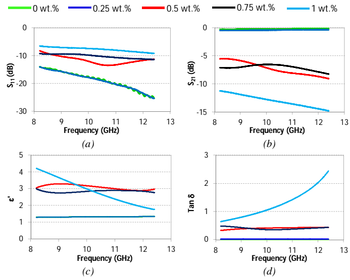
Fig. 5. (a) Reflection coefficients, (b) transmission coefficients from waveguide, (c) Permittivity and (d) \text{Tan } \delta extracted from the waveguide measurements for different carbon fiber loads.
