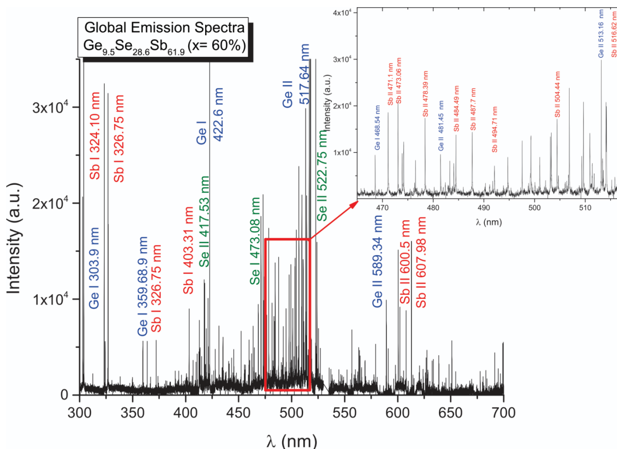
FIG. 4. Typical emission spectrum of the (\text{GeSe}_2)_{40}(\text{Sb}_2\text{Se}_3)_{60} laser ablation plasma at 6 mm from the target (25 ns gate delay, 2 \mu\text{s} gate width)
