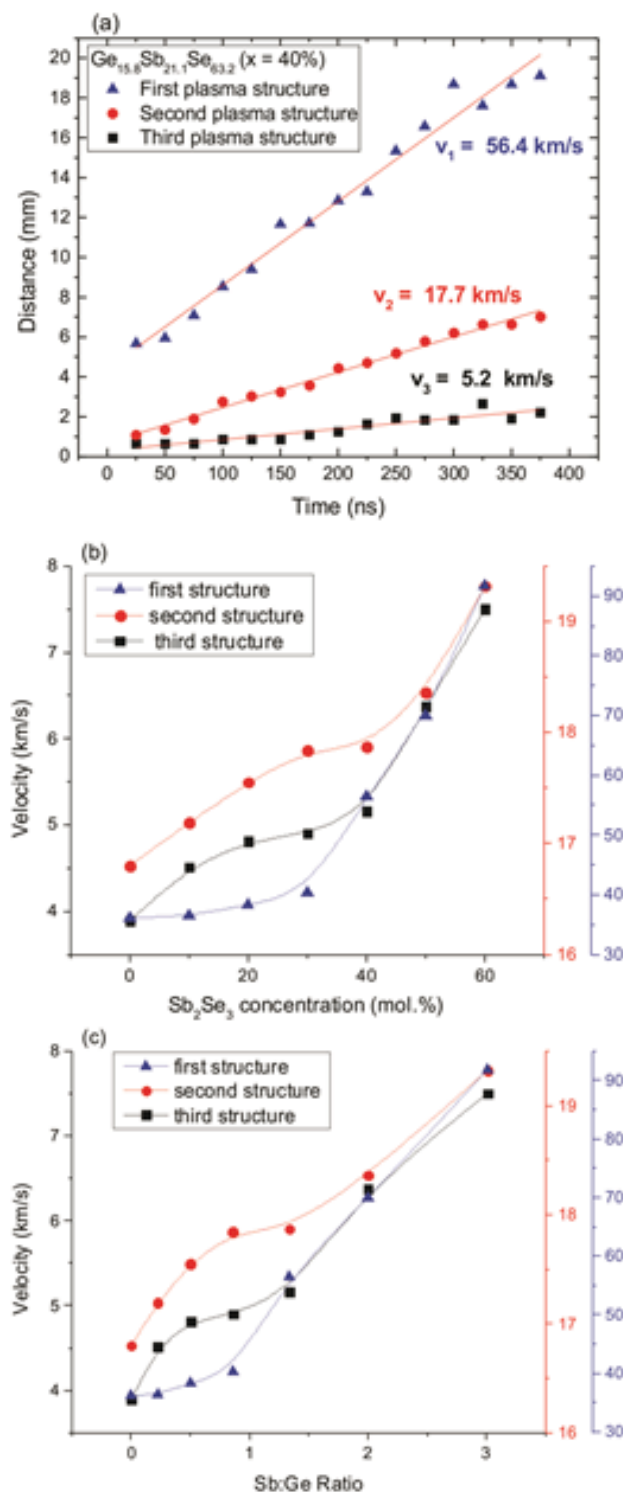
FIG. 3. The maximum emission point displacement in time (a) and the dependence between the expansion velocity on (b) \text{Sb}_2\text{Se}_3 concentration and (c) Sb:Ge ratio
