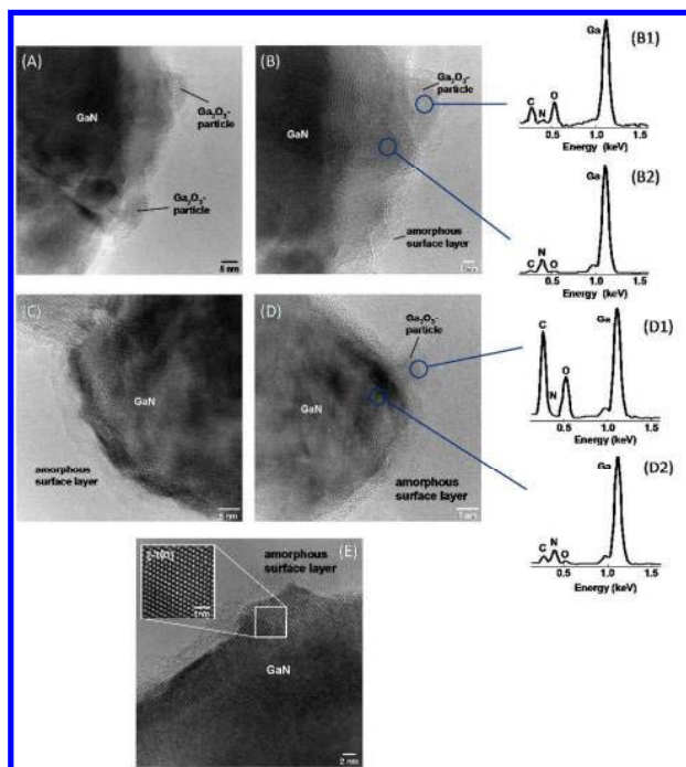
Figure 3. HRTEM images of “GaN” (A,B) and “GaN/NH 3 ” (C,D,E); inset in (E) FFT filtered image of the matrix near to the surface of “GaN/NH 3 ” specimen. Corresponding EDS spectra are shown in (B1, B2, D1, D2).
