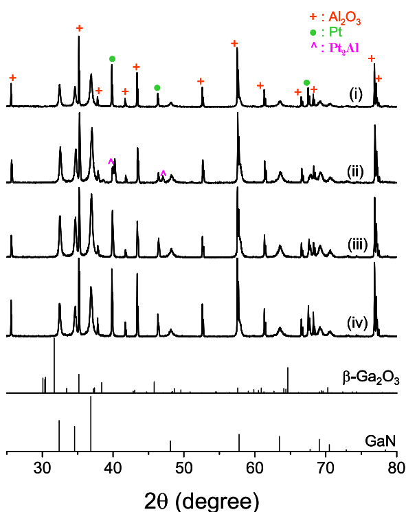
Figure 2. X-ray powder diffraction (XRPD) patterns of GaN layers on sensor substrates before and after gas sensing measurements: (i) and (ii) represent “GaN” coated sensor substrates before and after sensing measurement, respectively; (iii) and (iv) represent “GaN/NH 3 ” coated sensor substrates before and after sensing measurement. Here, it should be noted that XRD characterization done on the GaN coated sensor substrates before sensing measurement, specimen (i) and (iii), are different sensor samples than those after sensing measurements, specimen (ii) and (iv). Al 2 O 3
