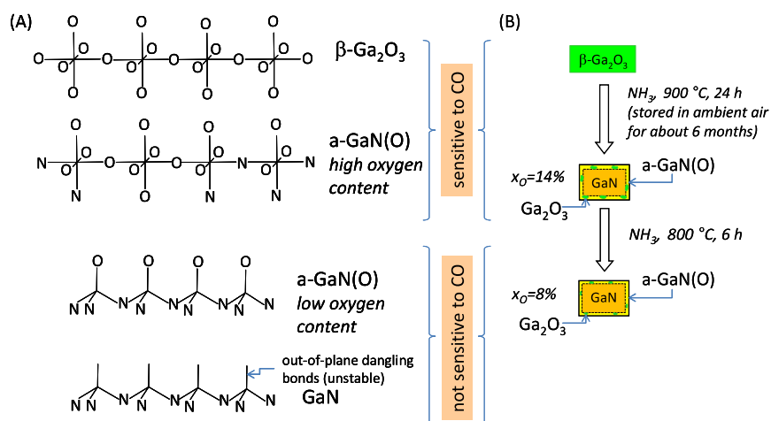
Figure 5. (A) Schematic representation of the local structure model representing the relationship between interaction of oxygen with GaN sensors and their sensitivity to CO. The tetrahedral coordination of Ga remains intact when a low amount of oxygen is incorporated. Interaction of oxygen with out-of-plane dangling bonds lead to the formation of amorphous gallium oxynitride with tetrahedral \text{a-GaN}(\text{O})\text{:GaN}_3\text{O} units that eliminate out-of-plane Ga-N bonds but do not influence the GaN bulk structure. Further increase of the oxygen amount leads to the formation of a distorted amorphous gallium oxynitride with octahedral \text{a-GaN}(\text{O})\text{:GaN}_2\text{O}_2 units. Complete substitution of N by O yields in distorted octahedral \text{GaO}_6 units. (B) Schematic representation of different stages of transformation process, from amonolysis of \text{Ga}_2\text{O}_3 to GaN followed by surface oxidation of as-synthesized GaN under air after storing for 6 months and finally re-treatment of “GaN” under ammonia at 800^\circ\text{C} for 6 h; \text{a-GaN}(\text{O}) represents amorphous gallium oxynitride layer formed due to surface oxidation.
