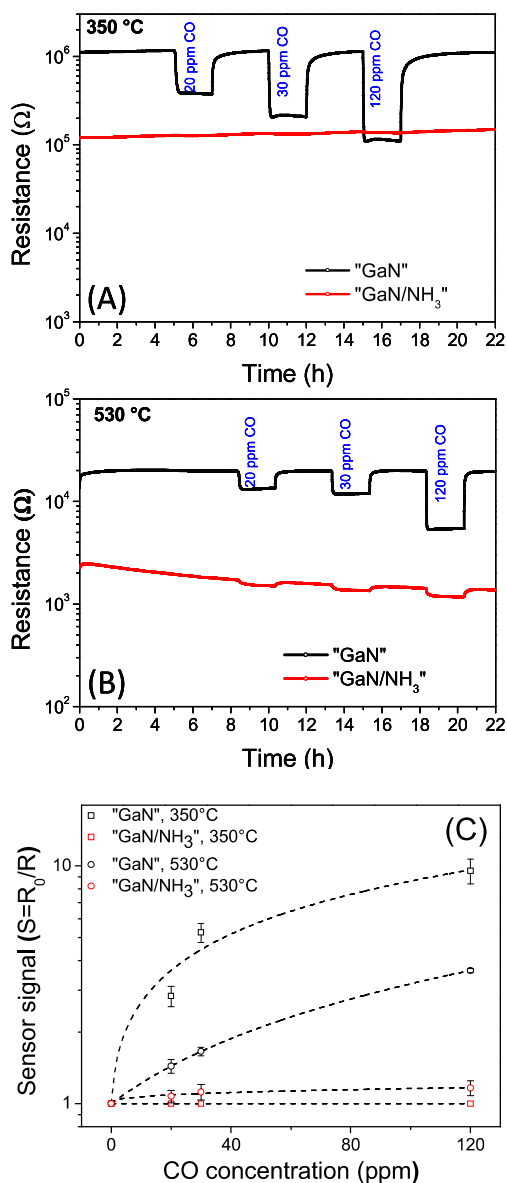
Figure 4. Transient response (A,B) and sensor signals ( S=R_0/R ) (C) of "GaN" and "GaN/NH 3 " sensors during exposure to CO (20, 30 and 120 ppm) in nitrogen at 350 °C and 530 °C; R_0 is baseline resistance whereas R is the resistance under different CO concentrations. In (c) the experimental points averaged over three measurements are fitted with a function S=1+aC^b where a=0.36, 0.03, 0.02 and b=0.66, 0.36, 1.00 for "GaN" sensors at 350 and 530 °C, and "GaN/NH 3 " sensors at 350 °C, respectively.
