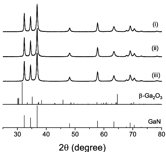
Figure 1. X-ray powder diffraction (XRPD) patterns of “GaN” (i), “GaN/N 2 ” (ii), and “GaN/NH 3 ” (iii) specimens (see Table 1). The diffraction patterns of β-Ga 2 O 3 (ICDD PDF No. 43-1012, monoclinic, space group C2/m, a = 12.23 Å, b = 3.04 Å, c = 5.80 Å) and GaN (ICDD PDF No. 50-0792, hexagonal, space group P6 3 mc, a = 3.18907 Å, b = 3.18907 Å, c = 5.1855 Å) are shown at the bottom.
