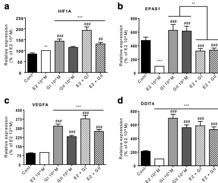
Fig. 7 Validation of differentially expressed genes corresponding to the HIF1 \alpha /EPAS1 community. MCF-7 cells were treated with vehicle (black), 10 -9 M E2 (white), 10 -5 M glyceollin I (light grey) and II (hard grey), or a combination of E2 and each of the glyceollins (hatched squares). The relative expression of HIF1 \alpha (a), EPAS1 (b), VEGFA (c) and DDIT4 (d) was assessed by real-time PCR and normalized to the expression of the housekeeping genes GAPDH and TBP. The results are expressed as the percentage of relative expression of each transcript obtained in E2-treated cells and are represented as the mean \pm SEM of 10 independent experiments. ** p -value <0.01 and *** p -value <0.001 with a Mann-Whitney test followed by Bonferroni correction for comparisons of the control vs the treatments. ## p -value <0.01 and ### p -value <0.001 with a Mann-Whitney test followed by Bonferroni correction for comparisons of E2 vs the other treatments
