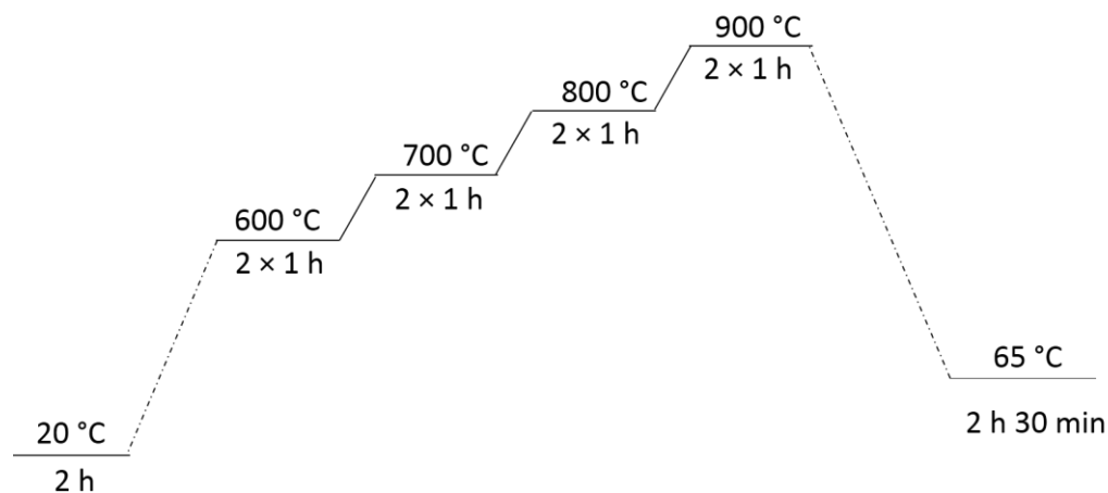
Fig.1. Thermal profile used in the neutron diffraction experiment under 5% \text{H}_2/\text{He} flow to convert the A-site disordered \text{Nd}_{0.5}\text{Ba}_{0.5}\text{MnO}_{3.8} phase to A-site ordered \text{NdBaMn}_2\text{O}_{5+\delta} phase. Heating and cooling rates are 10 °C min -1 .
