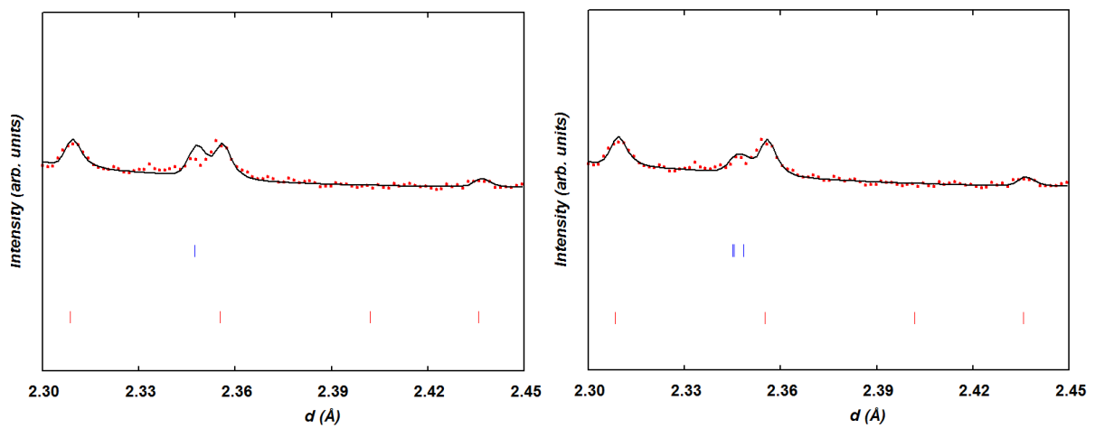
Fig. 4 Part of the NPD data collected at 20 °C for \text{Nd}_{0.5}\text{Ba}_{0.5}\text{MnO}_{3-\delta} comparing the fits at d \sim 2.35 Å (left) S.G. I4/mcm and (right) S.G. Imma ; lower markers relate to the hexagonal \text{BaMnO}_3 phase (S.G. P6_3/mmc ).
