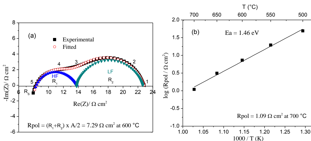
Fig. 12. Electrochemical performance of NdBaMn 2 O 6 symmetrical cell on CGO electrolyte: Nyquist impedance diagrams at 600 °C in air at OCV (numbers indicate the logarithm of the measuring frequency), (b) Arrhenius plot.
