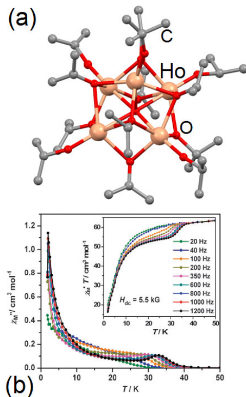
Figure 21. (a) Molecular structure of 28 . Hydrogen atoms are omitted for clarity. (b) Temperature dependence of the out-of-phase component of the magnetic susceptibility in an applied field of 5.5 kOe. In inset, Temperature dependence of the in-phase component of the magnetic susceptibility in an applied field of 5.5 kOe. The applied frequencies ranged from 20 to 1200 Hz. Adapted from ref [103].
