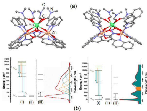
Figure 23. (a) Molecular structures of [\text{YbZn}_4(\text{L}^{22})_4(\text{py})_4(\text{DMF})_4]^{3+} (left) and [\text{YbZn}_4(\text{L}^{22})_4(\text{iqn})_4(\text{DMF})_4]^{3+} (right). Hydrogen atoms, triflate anions and solvent molecules of crystallisation have been omitted for clarity. (b) Correlations of the different set of data for the energy levels of the ^2\text{F}_{7/2} ground state multiplet obtained from dc fit (i) ac fit (ii) and luminescence spectra (iii) for 31 (left) and 32 (right). Adapted from ref [124].
