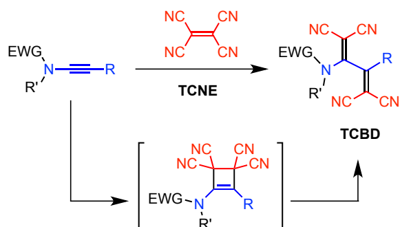
Scheme 1. Reaction between an ynamide and TCNE.
