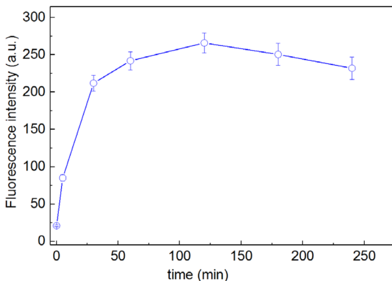
Figure 10. Photo-generation of ^{\circ}\text{OH} -radical under UV irradiation on \text{TiO}_2 deposited on GFT. The measurement were carried out in triplicate, error bars=5%.
