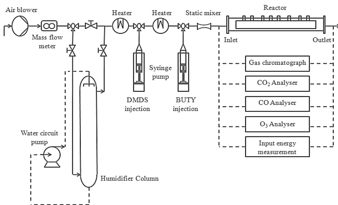
Figure 3. Experimental setup.
