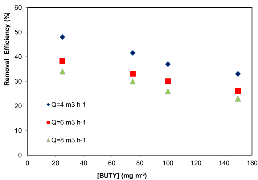
Figure 4. Removal efficiency (RE) of BUTY with inlet concentration at different flow rates (Process tested: Photocatalysis, UV intensity= 20 W m -2 , RH = 50 %).
