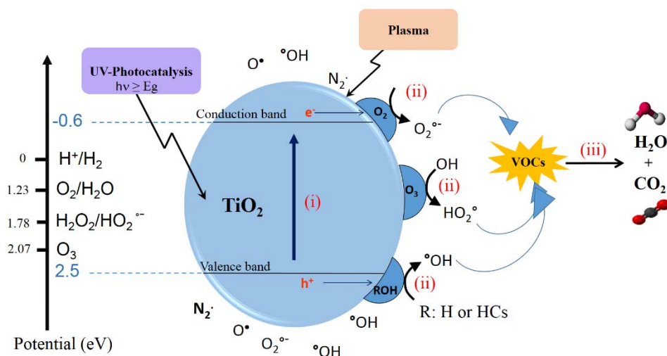
Scheme 1. Suggested mechanism for VOCs removal under UV/TiO 2 /O 3 combined processes.
