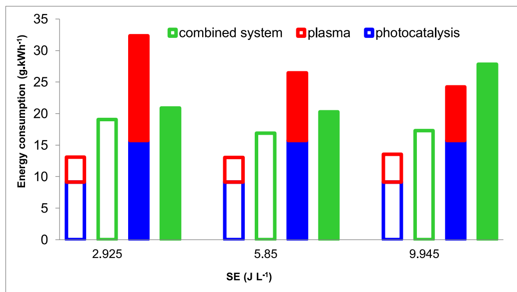
Figure 11. Variation of Energy Consumption (EC) vs SE at different configurations of tested processes ( Q=4 \text{ m}^3 \text{ h}^{-1} , [Pollutant] = 45 ppm) (dark color: butyraldehyde; light color: DMDS)
