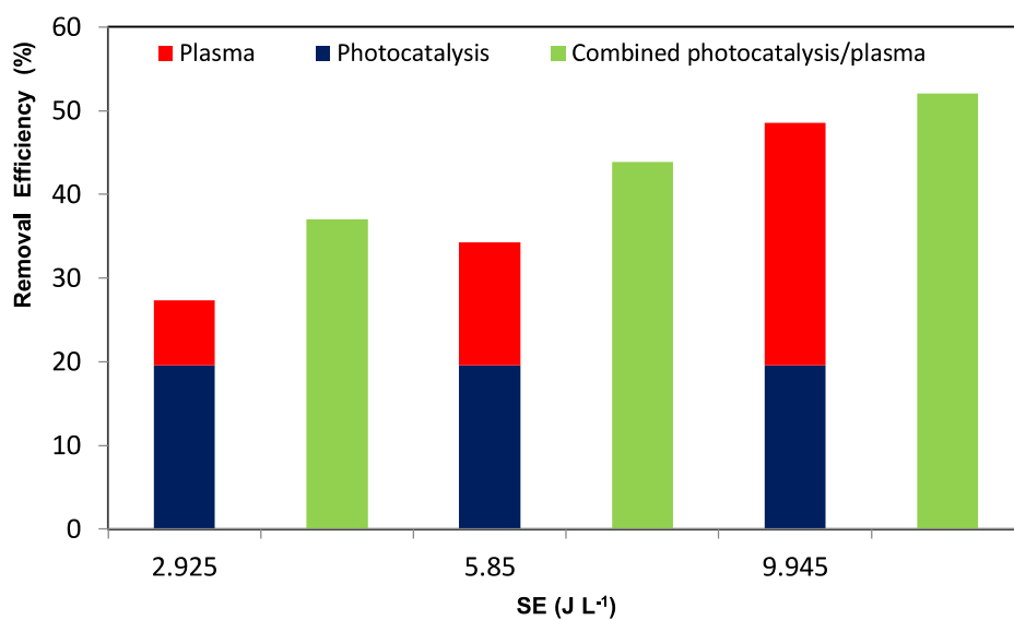
Figure 5. BUTY removal efficiency at different SE when applying DBD plasma, photocatalysis and their combination: Evidence for synergetic effect ( Q=4 \text{ m}^3 \text{ h}^{-1} , [\text{BUTY}] = 45 \text{ ppm} , \text{RH} = 50\% ).
