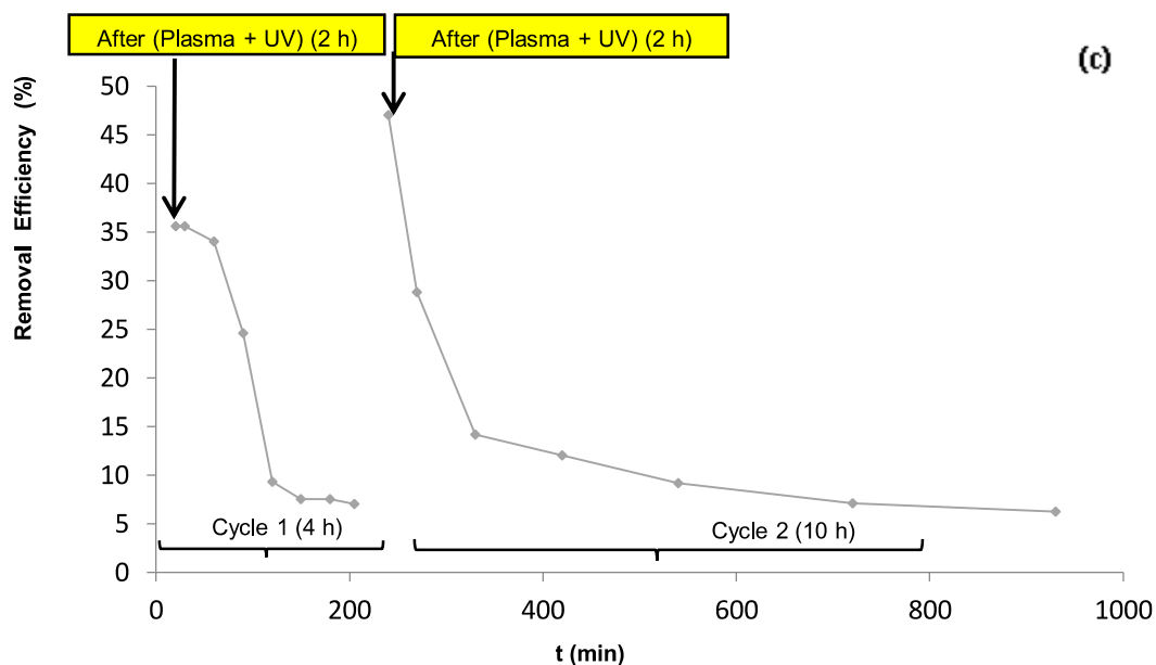
Figure 9. Variation of BUTY removal efficiency as function of time showing catalyst poisoning during the photocatalytic process ( Q = 1 \text{ m}^3 \text{ h}^{-1} , [Mixture] = 45 ppm, RH = 5%) with different process of regeneration: (a) process regeneration: photocatalysis, (b) process regeneration: DBD-plasma, (c) process regeneration: DBD-plasma combined with photocatalysis.
