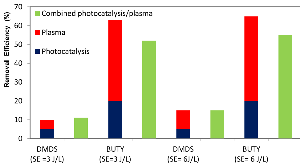
Figure 8. Variation of the removal efficiency of DMDS and BUTY in mixture (50%-50%) with SE using the three processes ( Q=4 \text{ m}^3 \text{ h}^{-1} , [\text{Mixture}] = 45 \text{ ppm} , \text{RH} = 50\% ).
