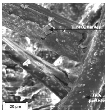
Figure 2. SEM imaging of TiO 2 deposited on GFT [38].
