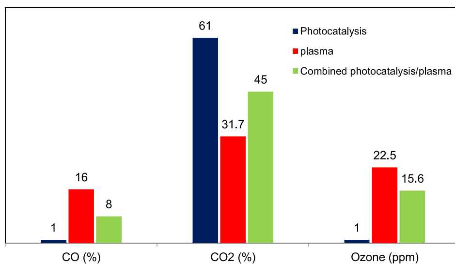
Figure 6. Variation of CO x selectivity (%) and the amount of ozone (ppm) when applying the three processes ( Q=4 \text{ m}^3 \text{ h}^{-1} , [\text{BUTY}] = 45 \text{ ppm} , \text{SE} = 9.945 \text{ J L}^{-1} , \text{RH} = 50\% ).
