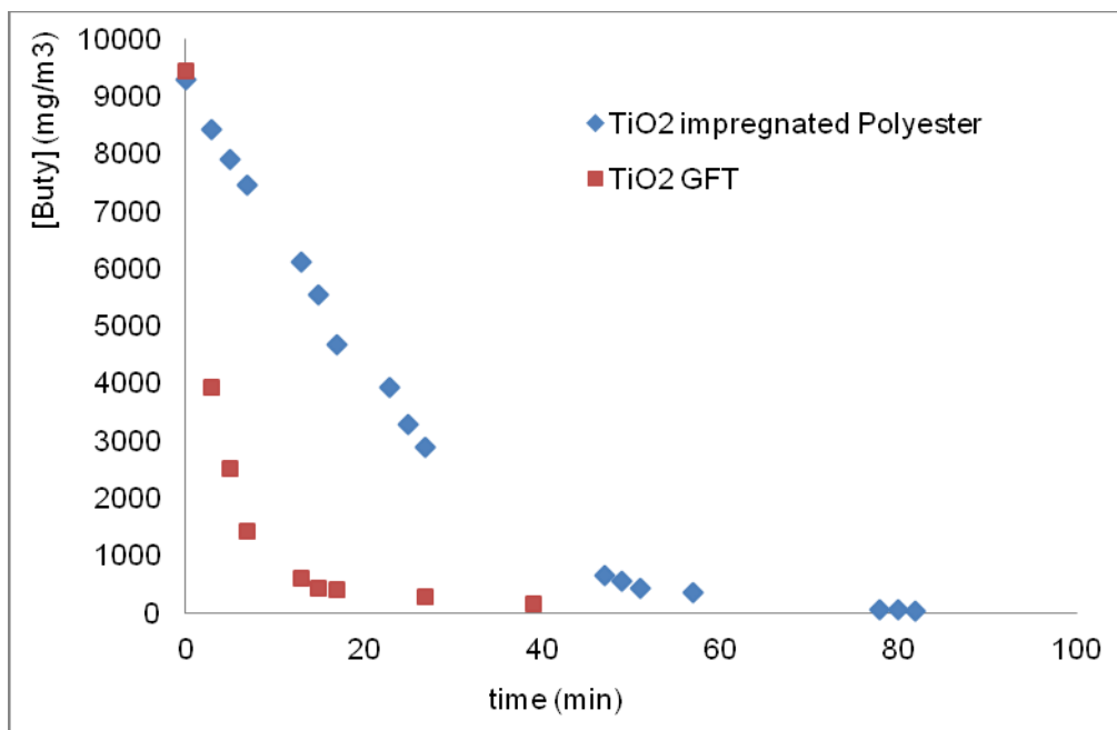
Figure 5a. Butyraldehyde photodegradation kinetics on GFT-TiO 2 and PES-TiO 2 samples under a Philips UV 9 W mercury lamp irradiation ( I=30W/m^2 ).
