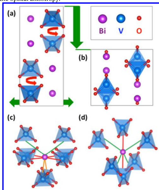
Figure 1. Schematic representation of the atomic structures of S_M - \text{BiVO}_4 (a) and Z_T - \text{BiVO}_4 (b). The structure filiation from S_M - and Z_T - \text{BiVO}_4 is highlighted with the green arrows (cell expansion along a and b, cell contraction along c) and the red arrows (rotation of \text{VO}_4^{3-} tetrahedra). The resulting local environments of bismuth atoms are given for S_M - \text{BiVO}_4 (c)
