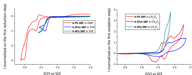
Figure 18. Cyclic voltammetry in reduction (left, recorded in DMF or THF + 0.1 M Bu 4 NPF 6 ) and in oxidation (right, recorded in CH 2 Cl 2 + 0.2 M Bu 4 NPF 6 ) of 4-Ph-SBF (red line), 4-5Pm-SBF (blue line) and 4-4Py-SBF (green line). The current is normalized at the first oxidation or reduction step. (Pt disk electrode Ø1 mm, 100 mV/s).
