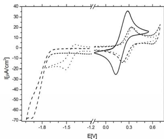
Fig. 6 Cyclic voltammograms of complexes 6 (dashed line) and 7 (dotted line), recorded in \text{CH}_2\text{Cl}_2 containing 0.1 \text{ M } n\text{-Bu}_4\text{N}^+\text{PF}_6^- at a vitreous carbon working electrode at 293 \text{ K} , v = 100 \text{ mVs}^{-1} , reference electrode \text{Ag}/\text{Ag}^+ , internal reference \text{Cp}_2\text{Fe}^{0/+} (solid line).
