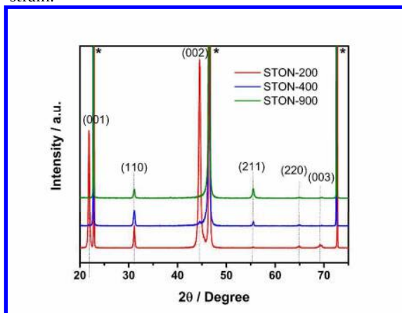
Figure 1. XRD \theta - 2\theta diffractogram patterns of different thickness of SrTaO 2 N films deposited on (001) Nb:STO substrate (indexation of films is made according to a pseudo-cubic cell) (* represents the (00L) diffraction peaks according to the substrate).
