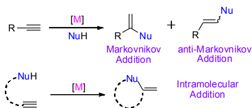
Scheme 1. Nucleophilic addition across a terminal alkyne.
