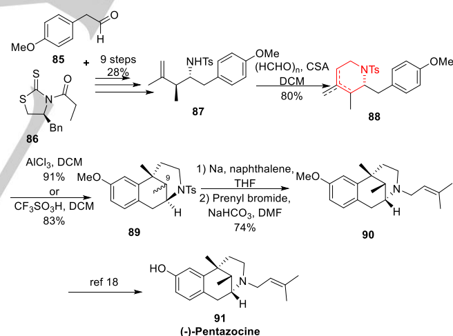
Scheme 19. She's formal total synthesis of (-)-Pentazocine.
