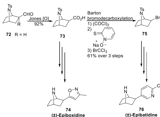
Scheme 16. Synthesis of ( \pm )-Epibatidine and ( \pm )-Epiboxidine from the common intermediate 72 .
