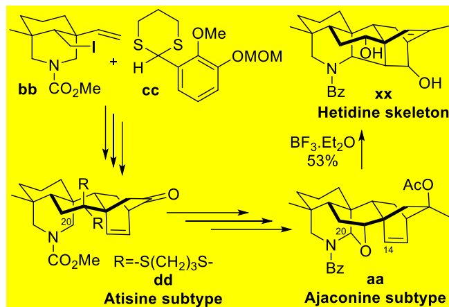
Scheme xx. Bioinspired synthesis of Hetidine skeleton via a late stage aza-Prins cyclization of Ajaconine subtype core.
