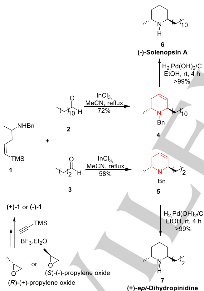
Scheme 2. Solenopsin A and epi -Dihydropinidine synthesis via aza-silyl-Prins cyclization.
