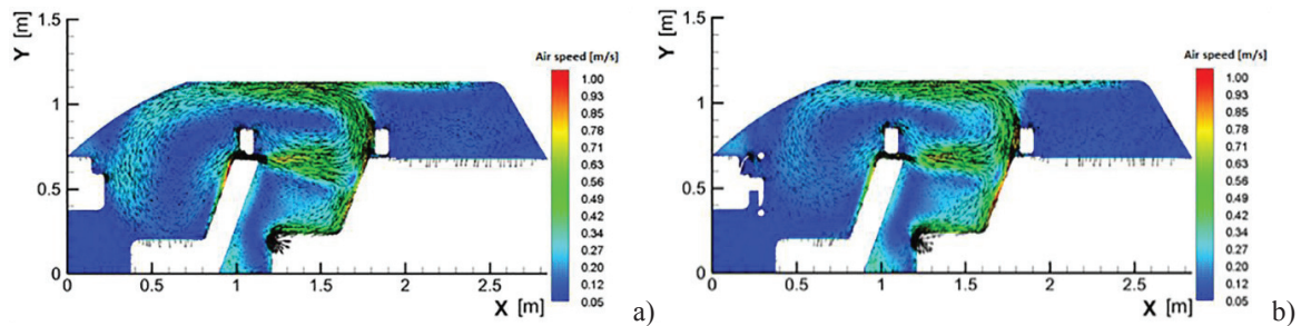
Fig. 5. Distributions of the velocity magnitude and of the in plane vectors: a). left part of the car; b). right part of the car
