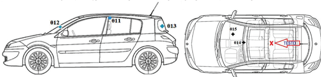
Fig. 1. a). K – type thermocouples at different passengers position b). monitored points in CFD model
