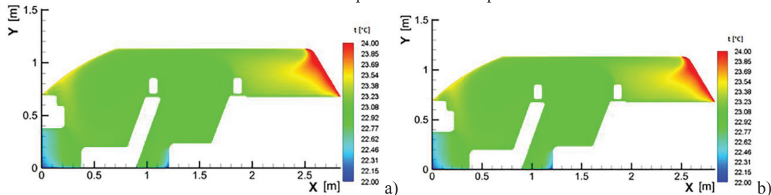
Fig. 6. Distributions of the air temperature: a)left side of the car; b)right part of the car
