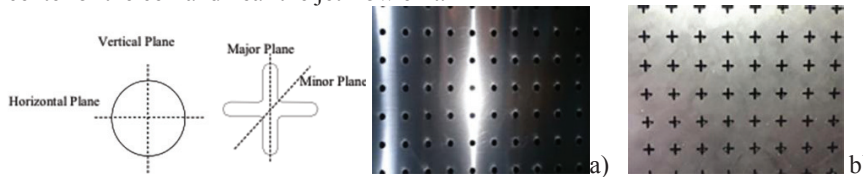
Fig. 1. Perforated panels with S=3.5De . a) Perforated panel with circular orifices, b) Perforated panel with cross orifices
