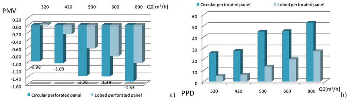
Fig. 4. Evolutions of the global thermal indexes from the ComfortSense data for several volumetric airflows. a) PMV, b) PPD
