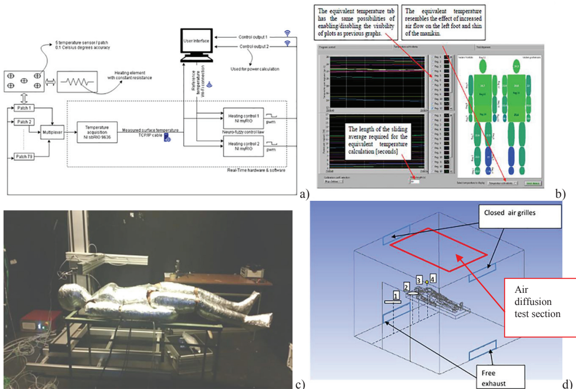
Fig. 2. a) Working principle of the thermal manikin, b) Map of the zones of the manikin, c) Photo of the thermal manikin prototype, d) Sketch of the climatic chamber with the positioning of the studied grilles and of the measurement points (1 – relative humidity, 2 – operative temperature probes, 3 – head of the thermal manikin, 4 – omnidirectional velocity probe)
