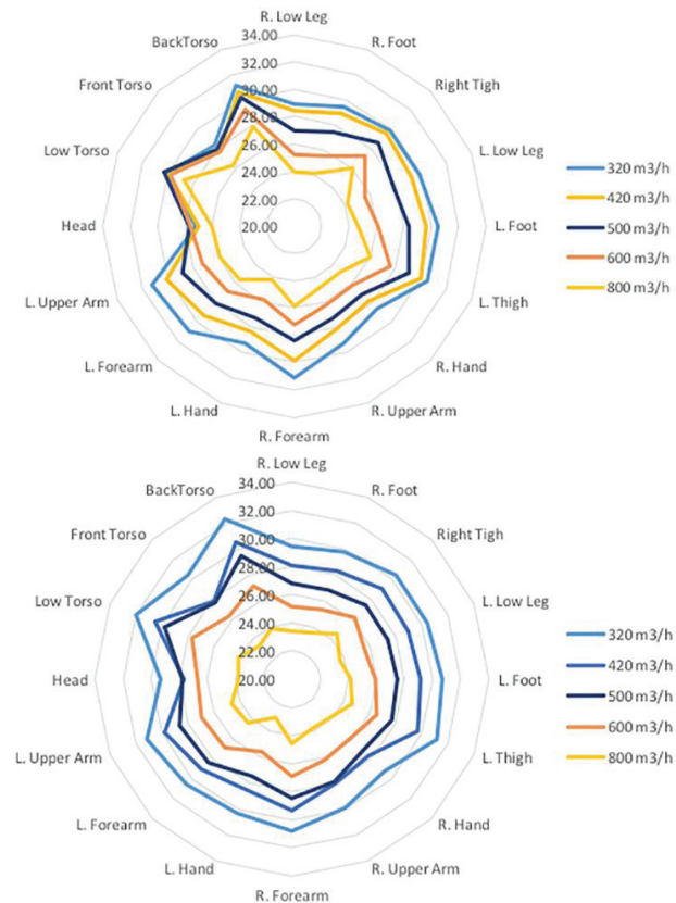
Fig. 5. Distributions of local t_{eq} obtained from the thermal manikin data for the two perforated panels
