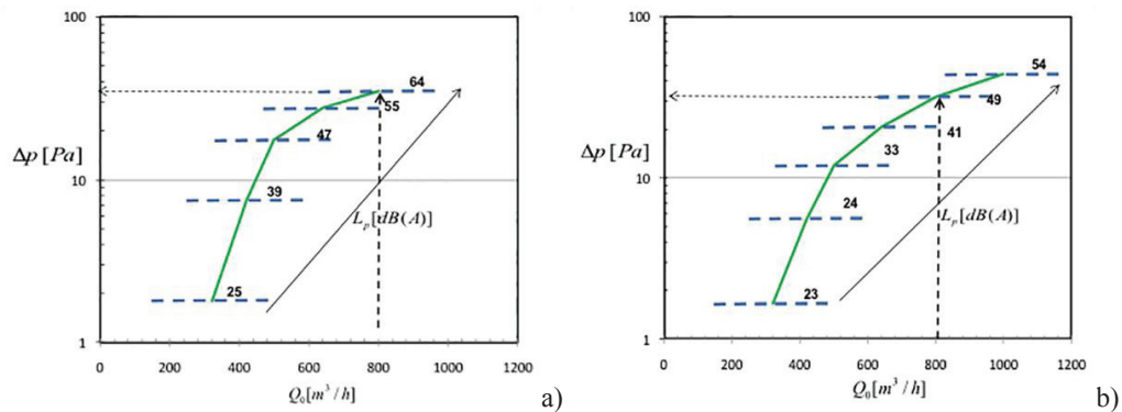
Fig. 3. Pressure losses and sound pressure levels of the perforated panels. a) circular orifices, b) lobed orifices
