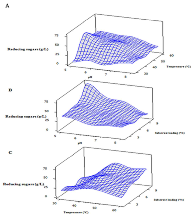
Figure. 4. Surface plots described by the proposed model showing the interactive effects of various parameters on reducing sugars production after enzymatic hydrolysis of hydrothermal pretreated potato peels residues
