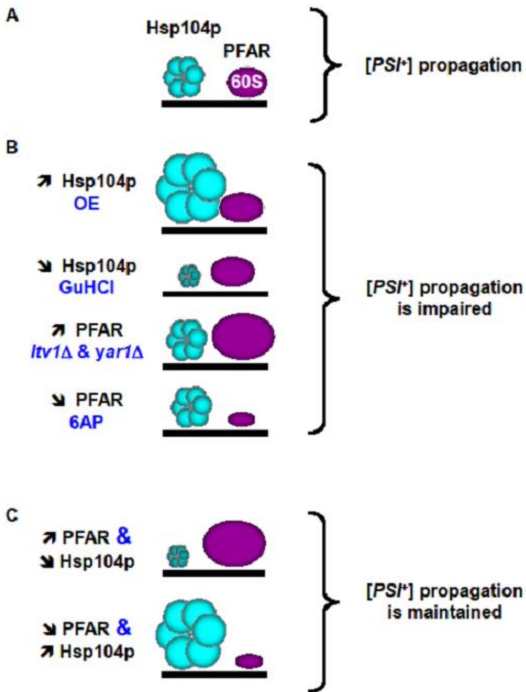
Figure 2. Interplay between protein folding activities of Hsp104p and ribosome in modulating [PSI^+] propagation (adapted from 6 ). A - Hsp104p and PFAR both participate in [PSI^+] propagation. B - [PSI^+] propagation is affected by enrichment or inhibition of Hsp104p
