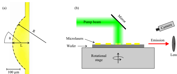
Figure 1. (a) A photograph with an optical microscope (top view) in real colors of a plano-concave microlaser. The width of the cavity is L = 125 \mu\text{m} and the radius of the concave boundary R = 250 \mu\text{m} in this example ( \rho = 1/2 ). The far-field observation angle is \theta . (b) Scheme of the optical characterization setup (side view, not to scale).
