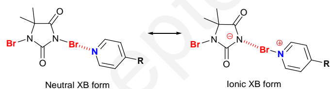
Scheme 4 Polarization on the XB adduct \text{DBH}\cdot[\text{Py}-\text{R}] .
