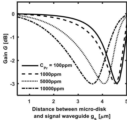
Fig. 13. Optical gain G as a function of distance g_s between micro-disk and signal waveguide for different praseodymium concentrations. The input pump power is P_{\text{in}}^{\text{pump}} = 0.01 mW and the input signal power is P_{\text{in}}^{\text{signal}} = -30 dBm.
