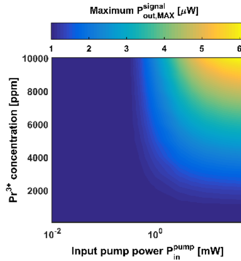
Fig. 12. Maximum output signal power P_{\text{out,MAX}}^{\text{signal}} as a function of input pump power P_{\text{in}}^{\text{pump}} and praseodymium concentration C_{\text{Pr}} . The input pump power P_{\text{in}}^{\text{pump}} varies in the range 0.01 mW–50 mW and the praseodymium concentration C_{\text{Pr}} in the range 100 ppm–10 000 ppm. The input signal power is P_{\text{in}}^{\text{signal}} = -30 dBm.
