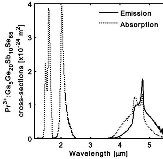
Fig. 6. Calculated emission and absorption cross-sections for the \text{Pr}^{3+}:\text{Ga}_5\text{Ge}_{20}\text{Sb}_{10}\text{Se}_{65} glass.
